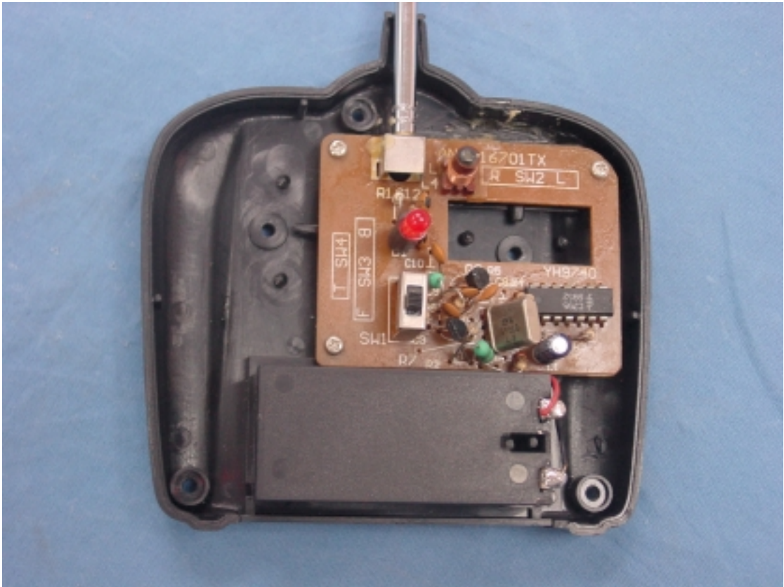
Figure 6 General Appearance of the PCB
