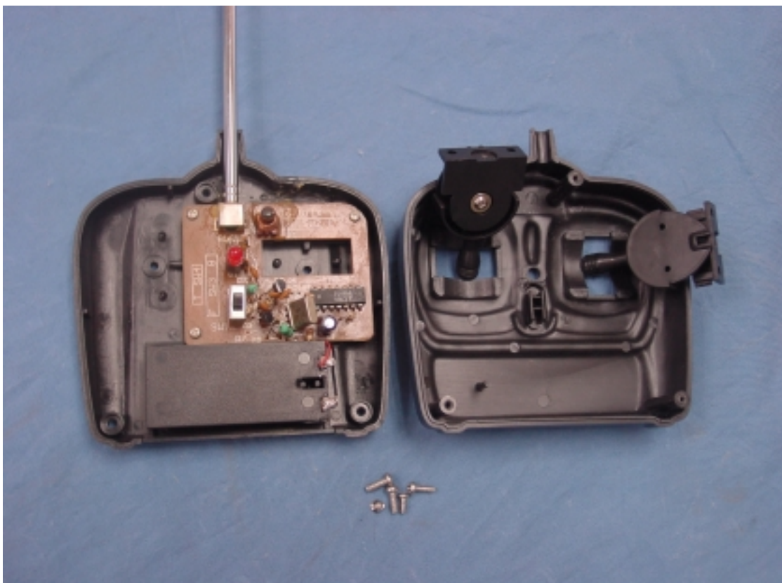
Figure 4 Cover Opened
