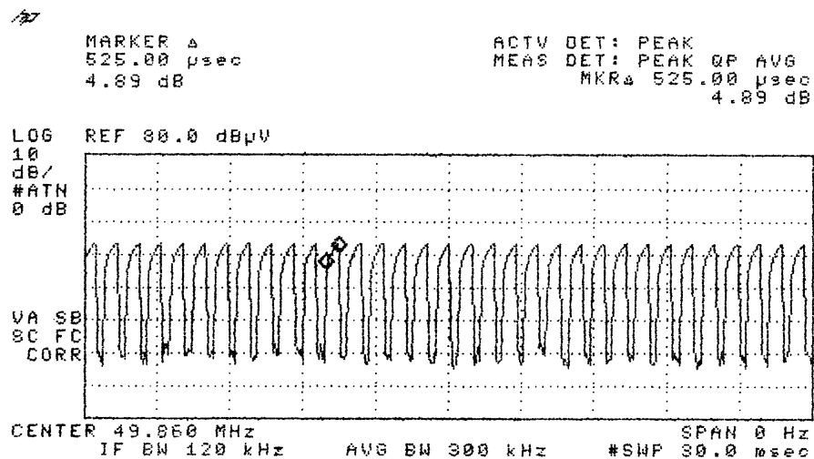
Figure B [Long and Short Pulse]
