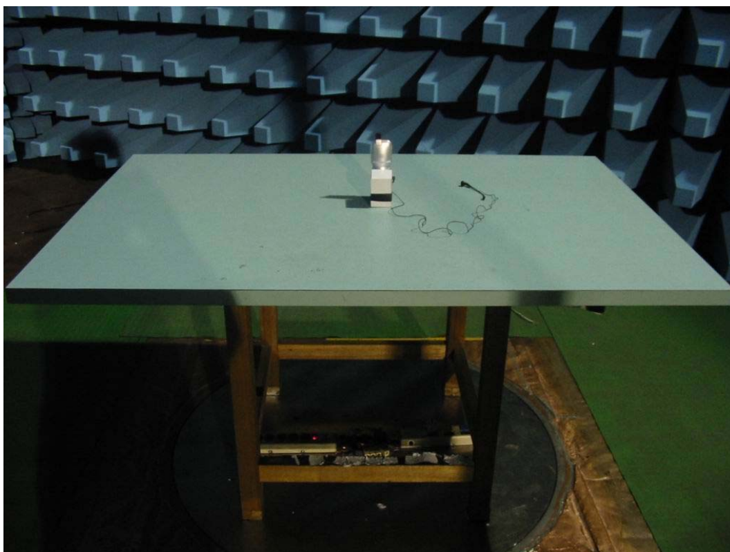
Rear View of the Test Configuration of Y-axis
