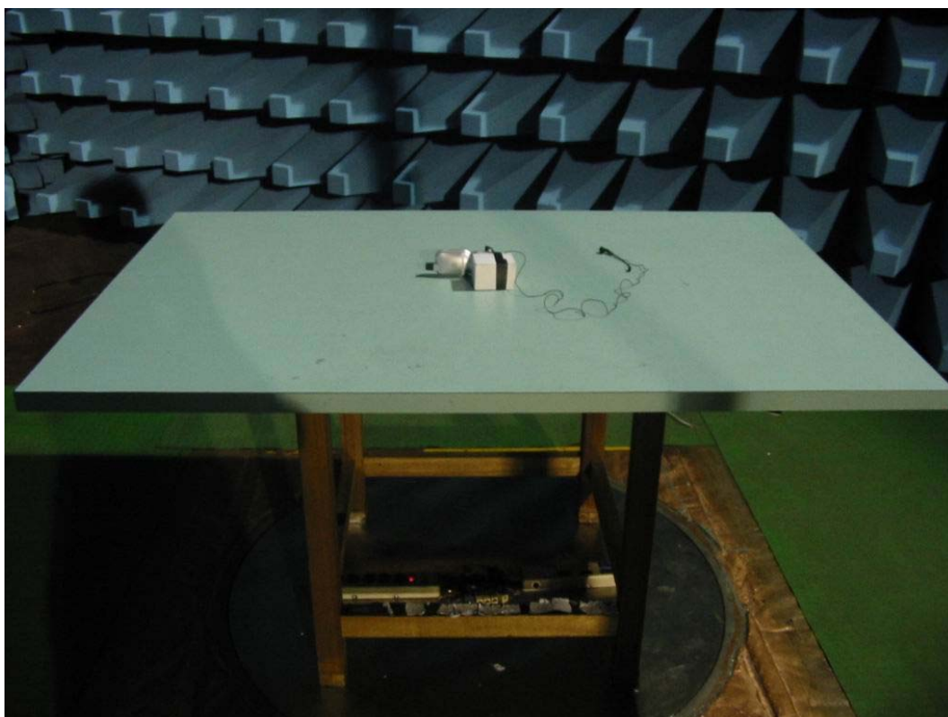
Rear View of the Test Configuration of Z-axis
