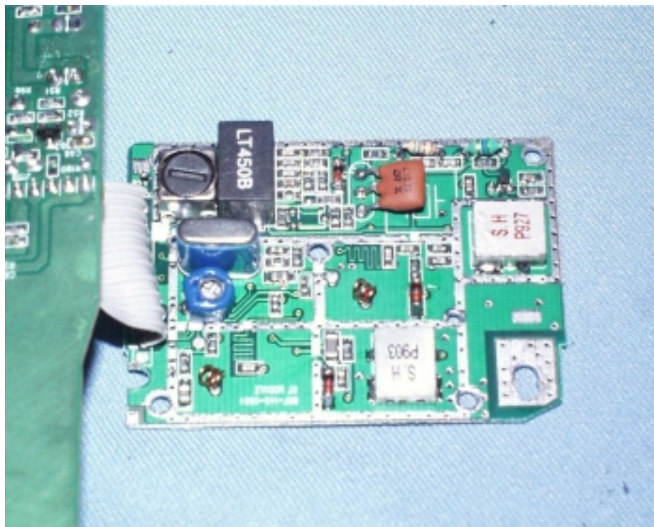
Base Oscillator PCB comp side
