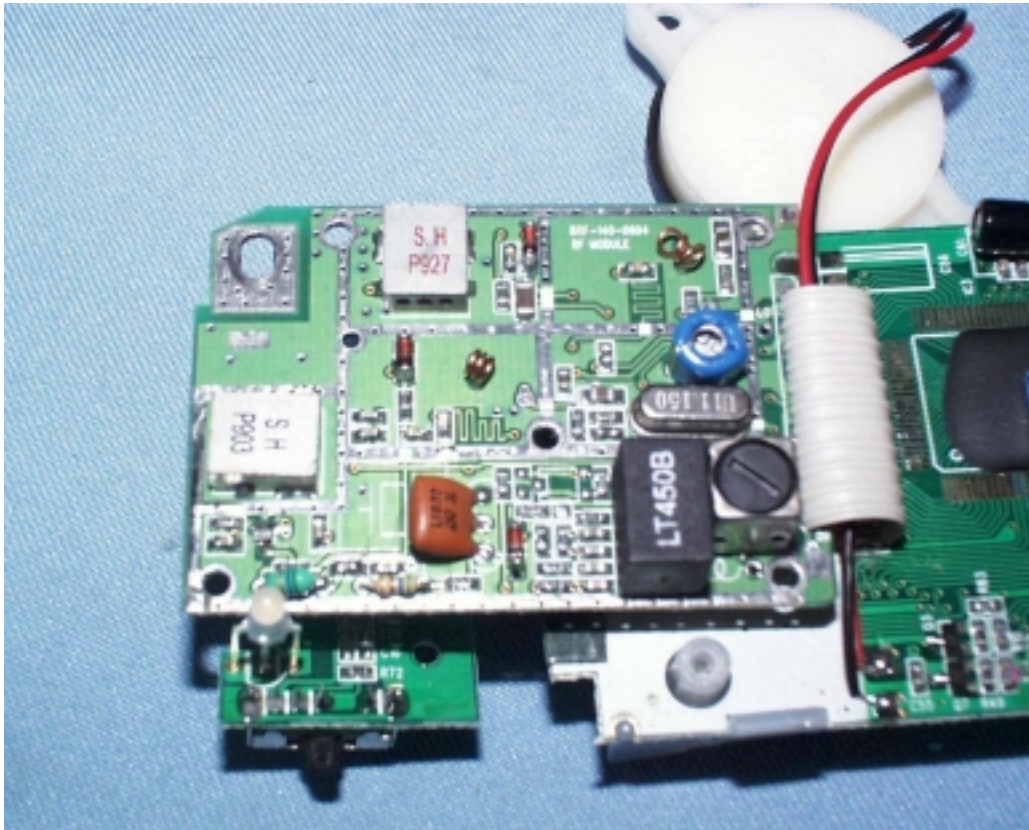
Handset Oscillator PCB solder side
