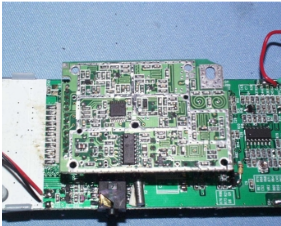
Handset Oscillator PCB solder side
