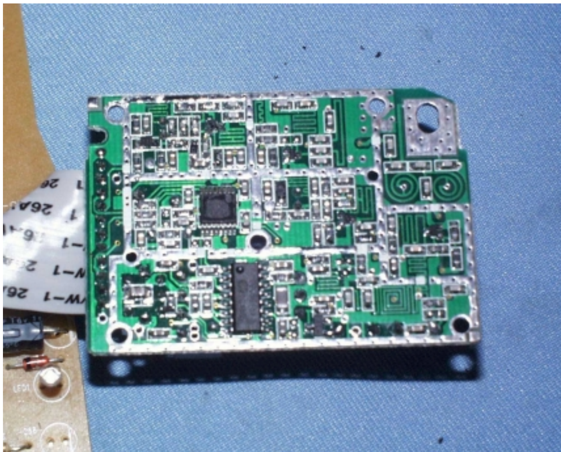
Base Oscillator PCB solder side
