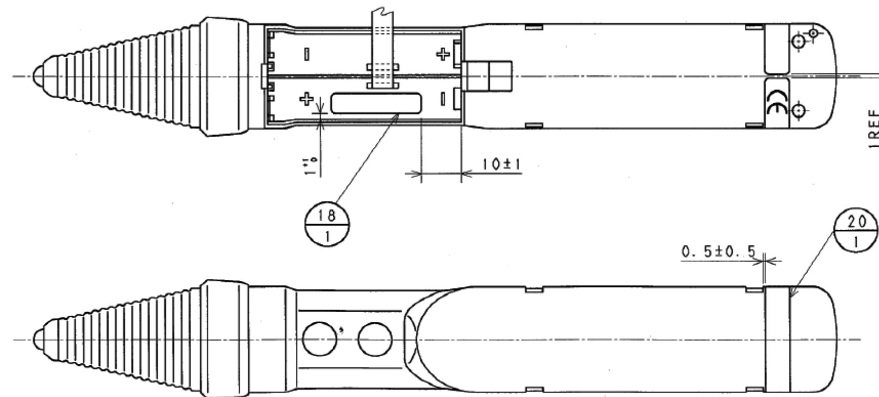
VIEW E
