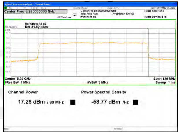
5290MHz_ax80_Ant A
