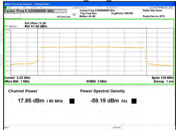
5530MHz_ac80_Ant A
