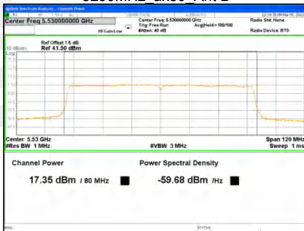
5530MHz_ac80_Ant B
