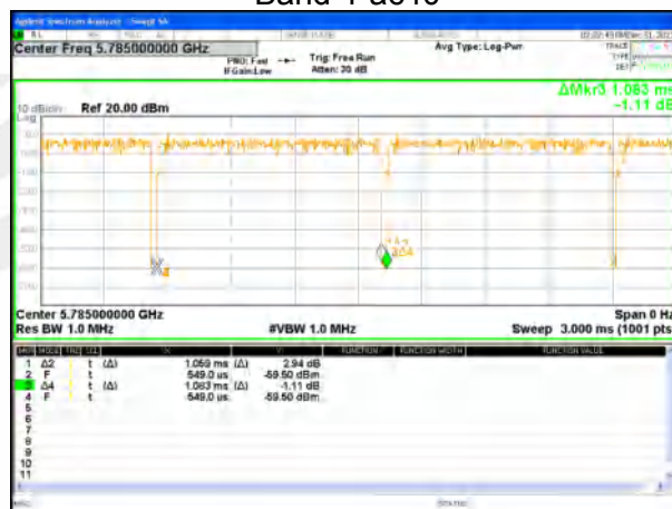
Band 4-ax20
