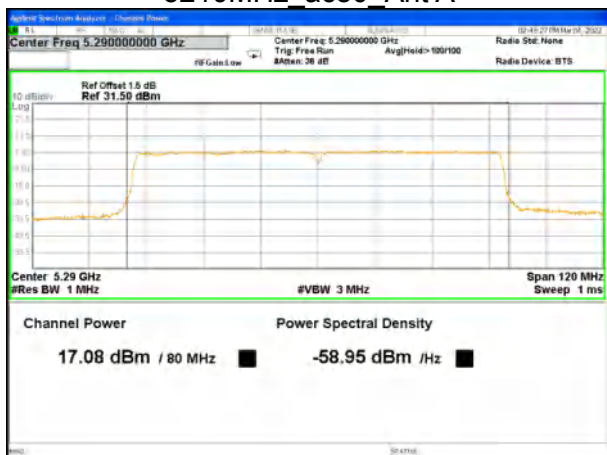
5290MHz_ac80_Ant A
