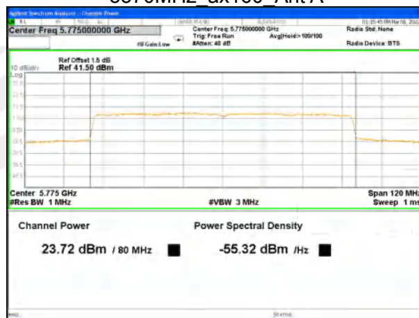
5775MHz_ax80_Ant A
