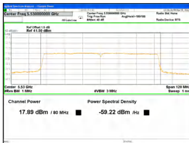
5530MHz_ax80_Ant A
