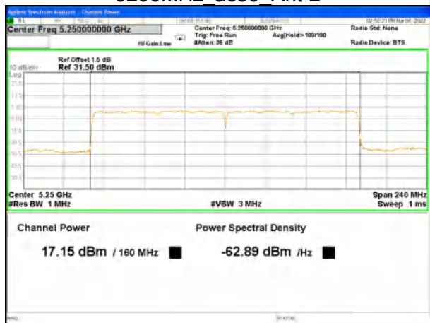
5250MHz_ax160_Ant B
