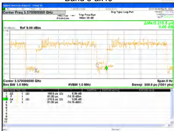
Band 3-ax160
