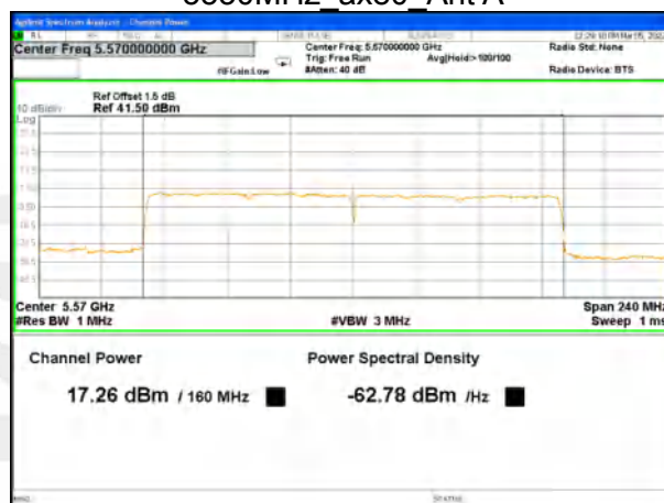
5570MHz_ax160_Ant A
