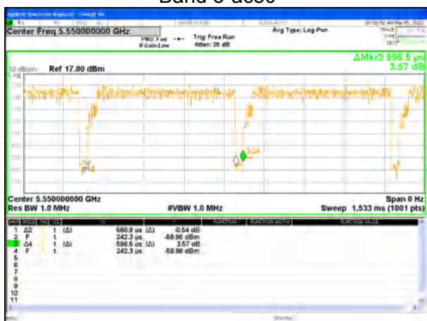
Band 3-ax40
