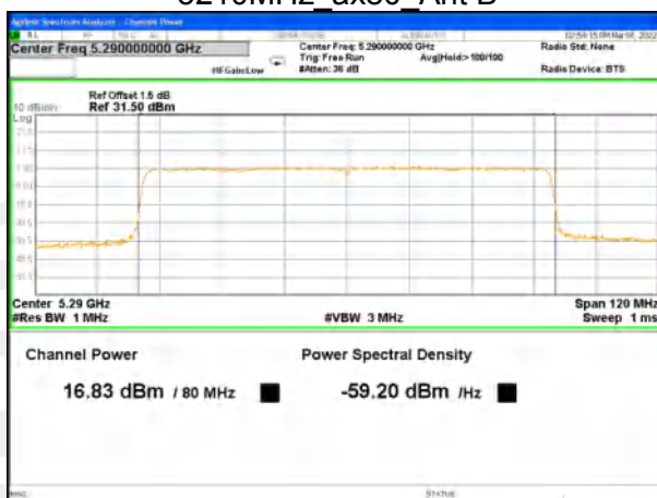
5290MHz_ax80_Ant B
