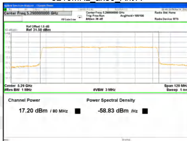
5290MHz_ax80_Ant A
