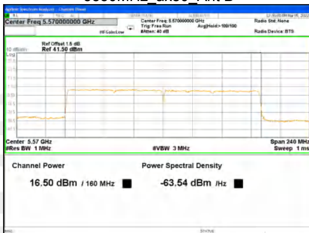
5570MHz_ax160_Ant B
