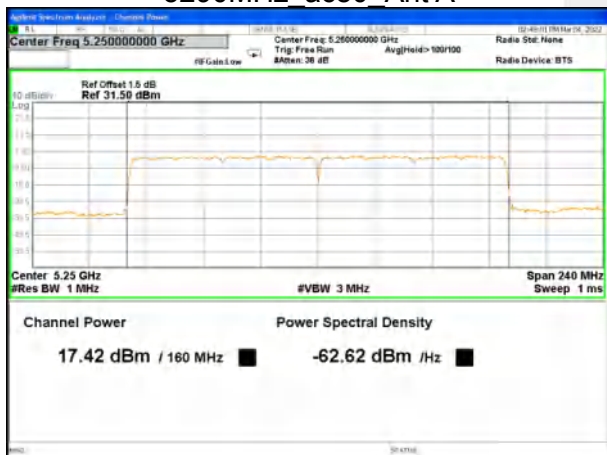
5250MHz_ax160_Ant A
