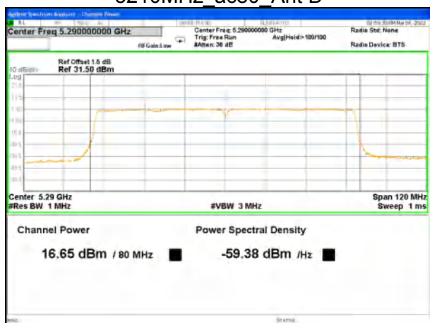
5290MHz_ac80_Ant B
