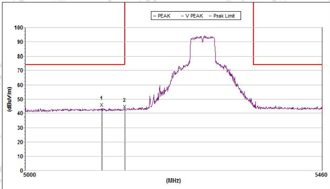
5270MHz Vertical
