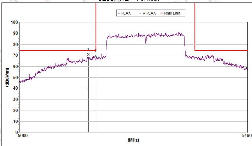
5250MHz Vertical
