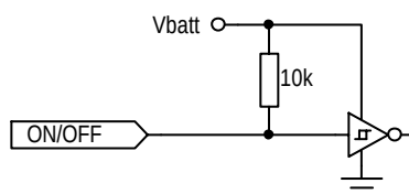
On/Off Input Circuit
