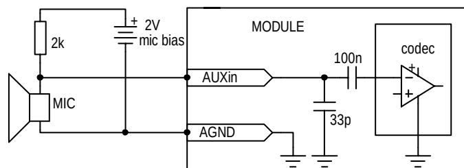
Auxiliary microphone input showing external biasing requirement
