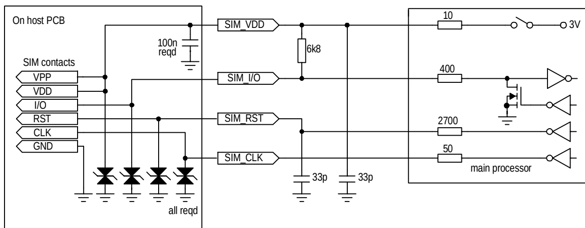
The SIM Interface circuit
