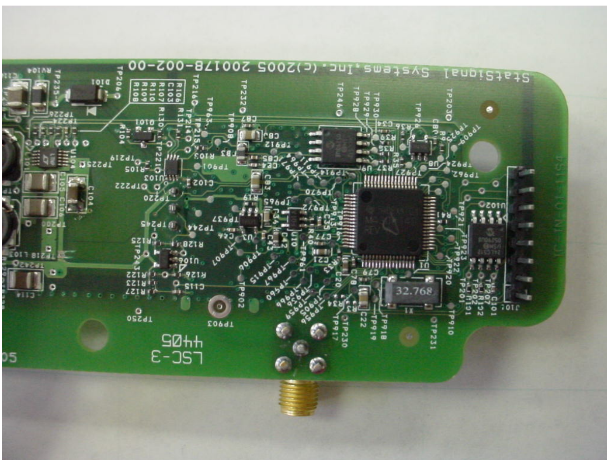
Photo Five – Internal Flip Side of RF Section
