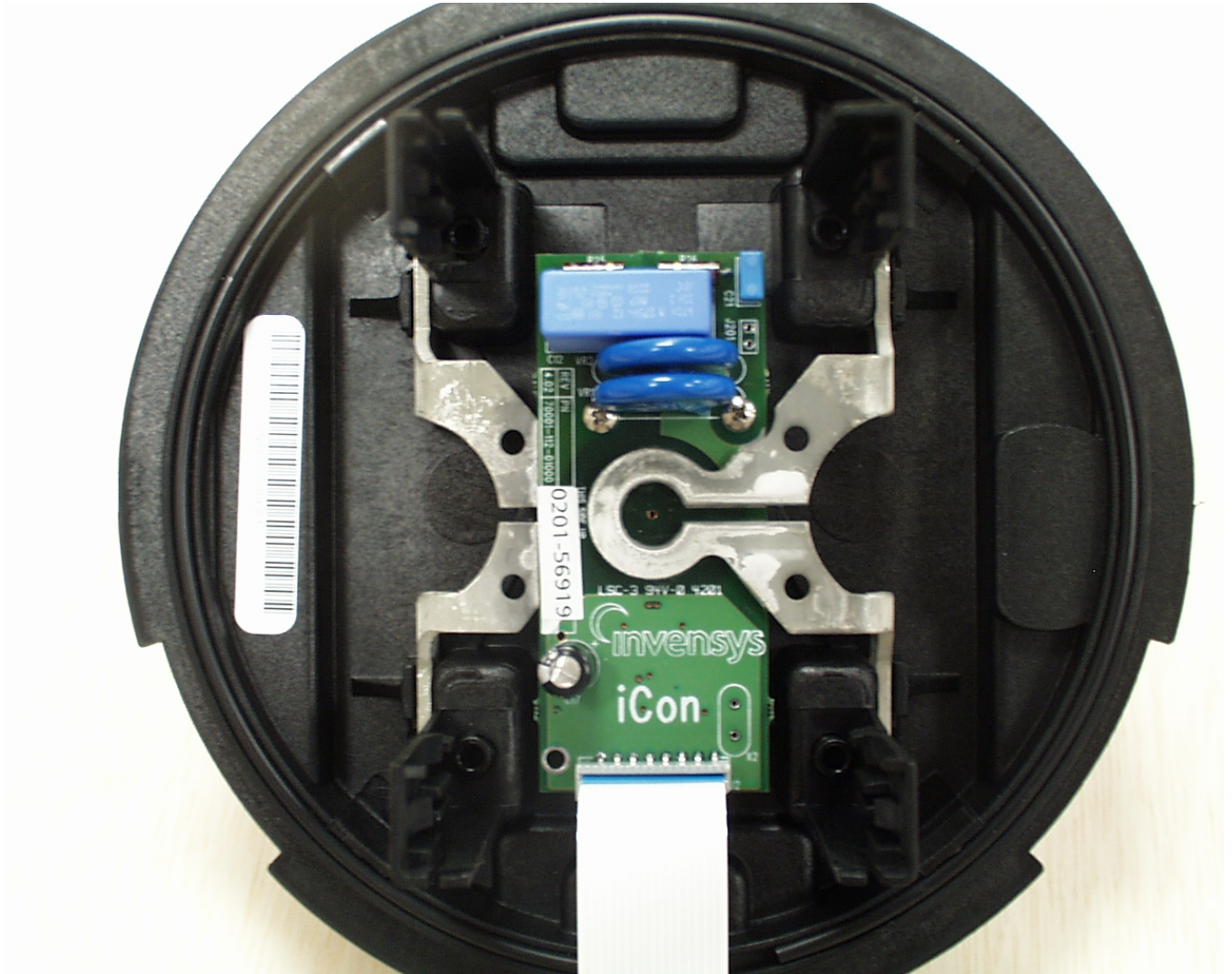
Internal Photograph 6: Icon metrology board
