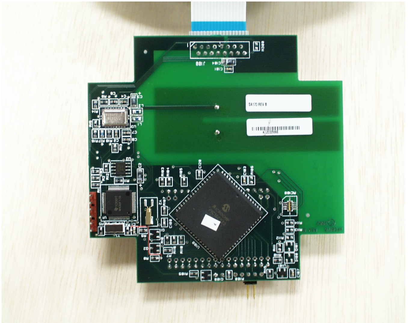
Internal Photograph 5: Bottom view of transmitter board
