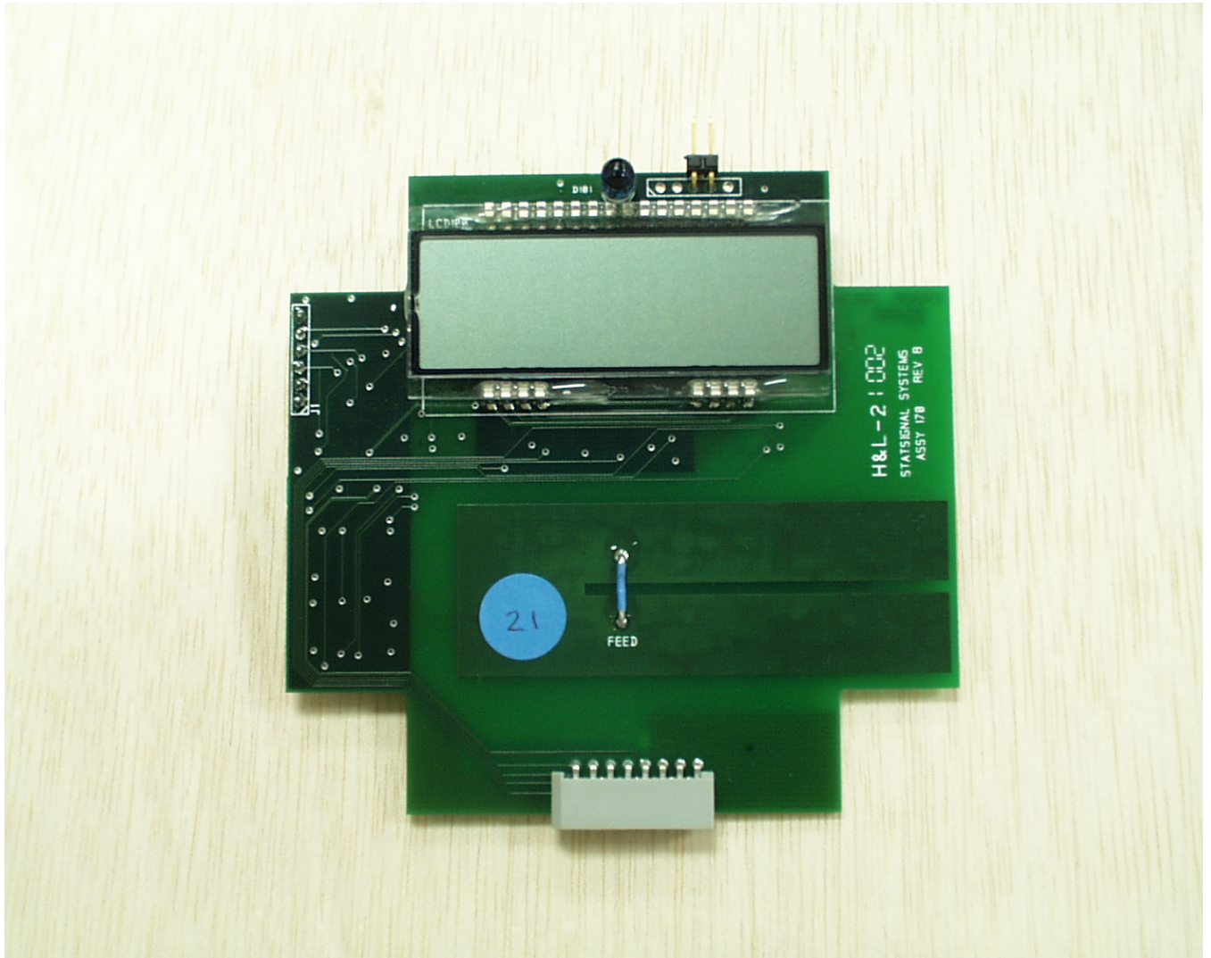
Internal Photograph 4: Top view of transmitter circuit board
