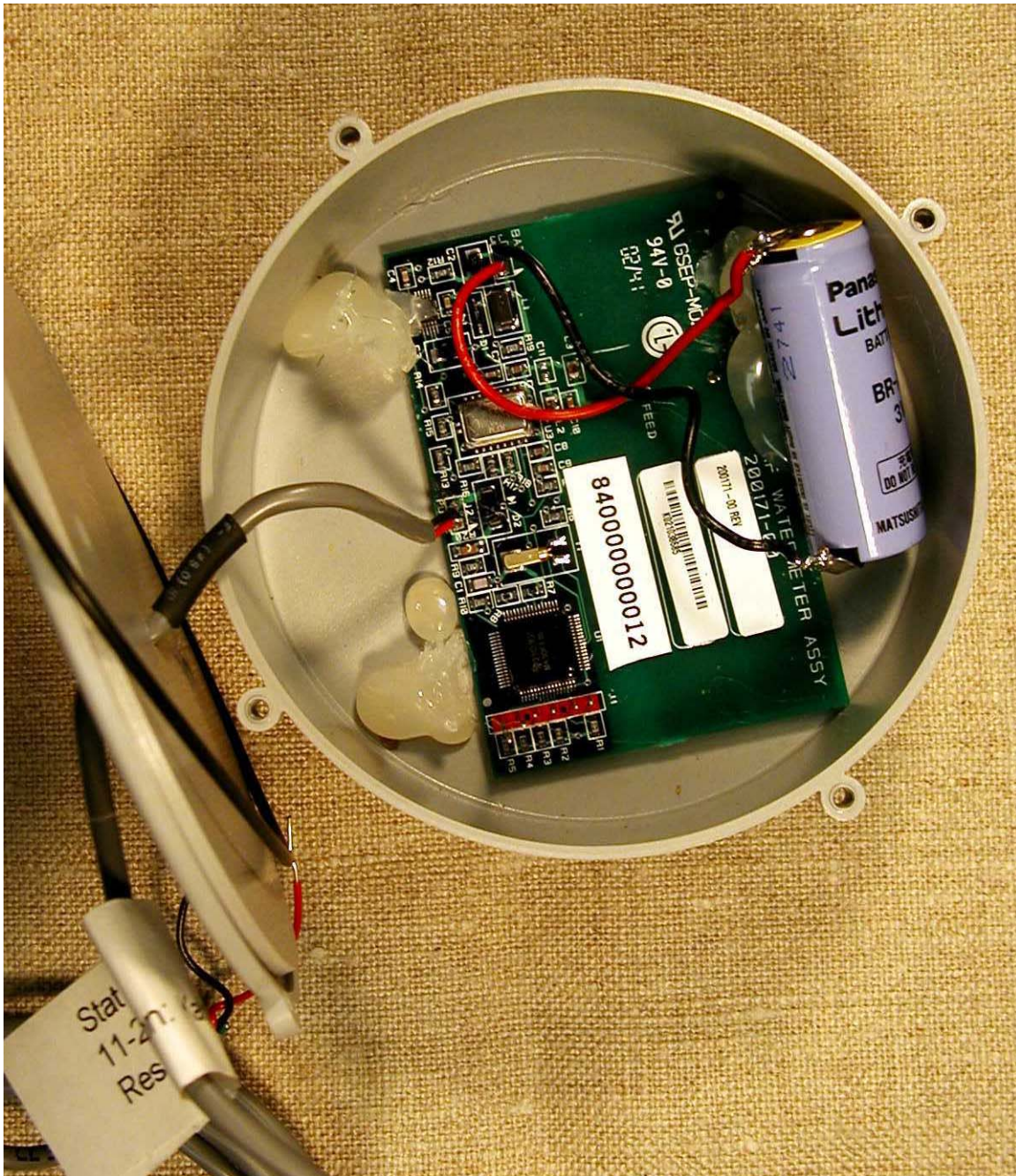
Internal Photograph 1: Enclosure with PCB
