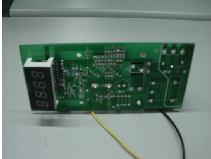
EUT- CONTROL BOARD PCB VIEW
