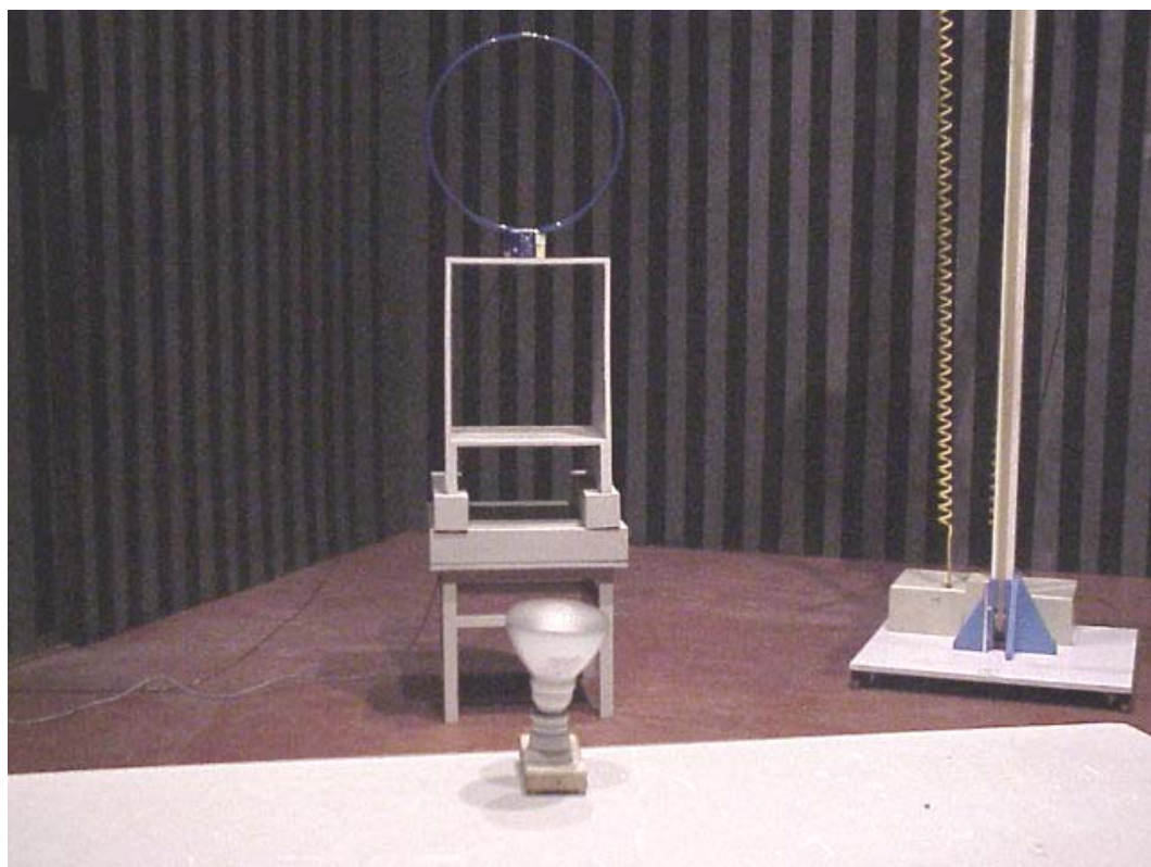
(RD SERIES)
