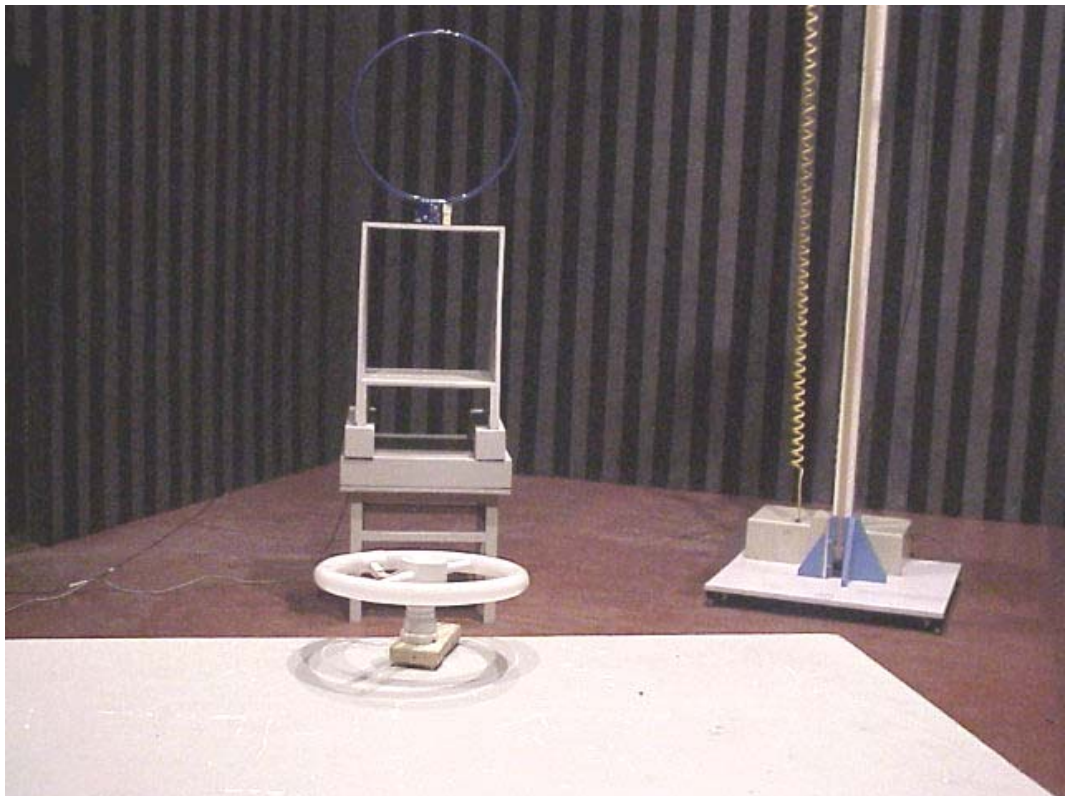
(T9D SERIES)
