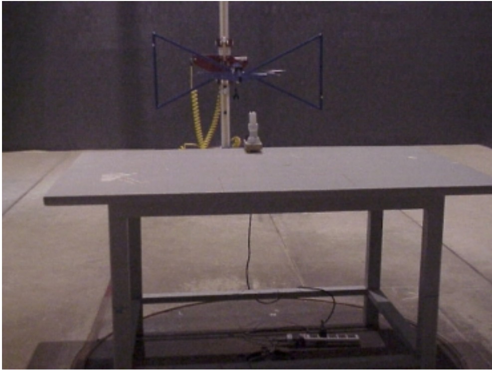
HORIZONTAL (M/N: FE-II SERIES)
