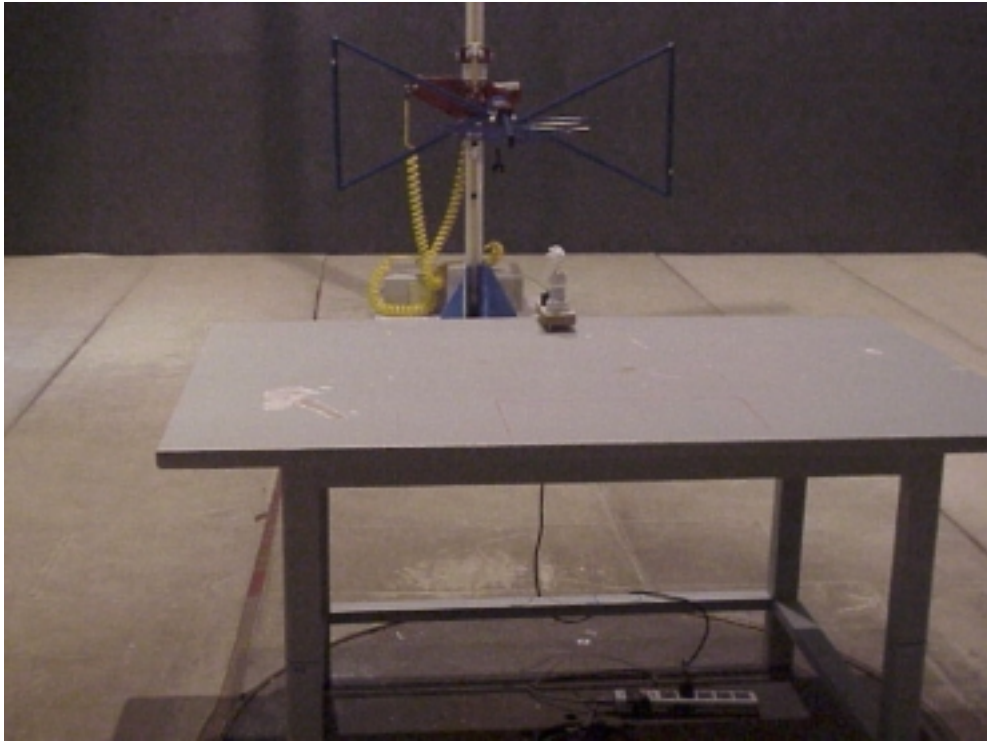
HORIZONTAL (M/N: FE-IIS SERIES)
