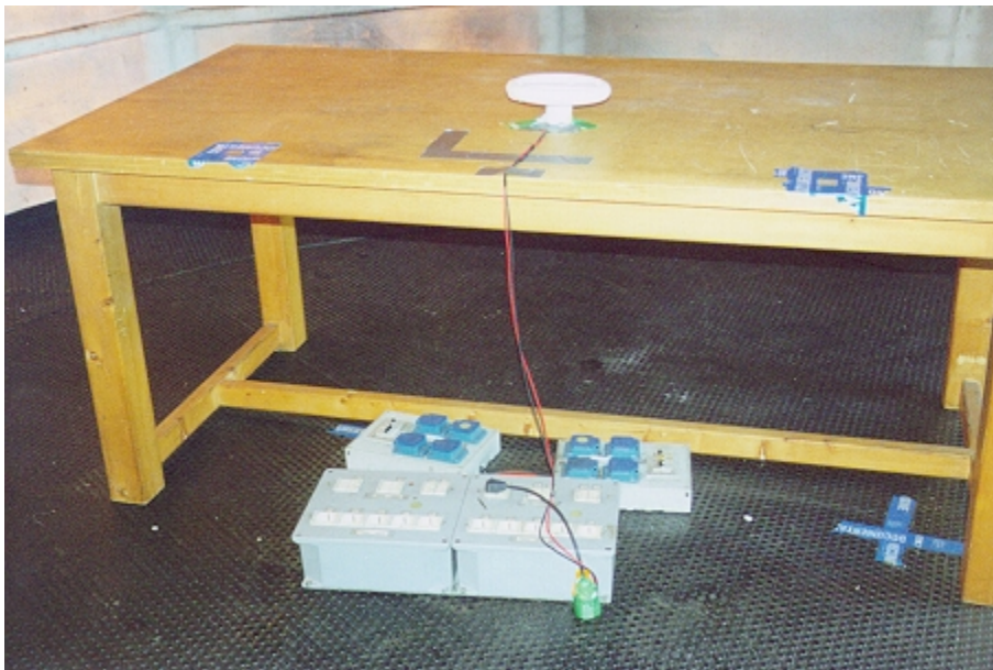
Radiated noise measurements test setup
