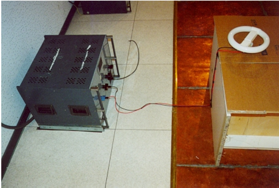
Conducted noise measurements test setup
