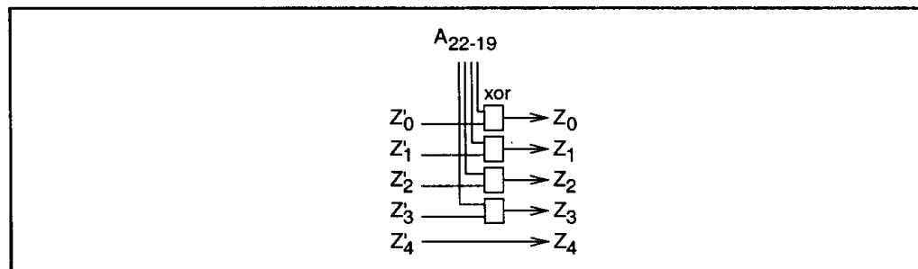
Figure 11.5: XOR operation for the 79-hop system. The 23-hop system is the same except for the Z'_4/Z_4 wire that does not exist.
