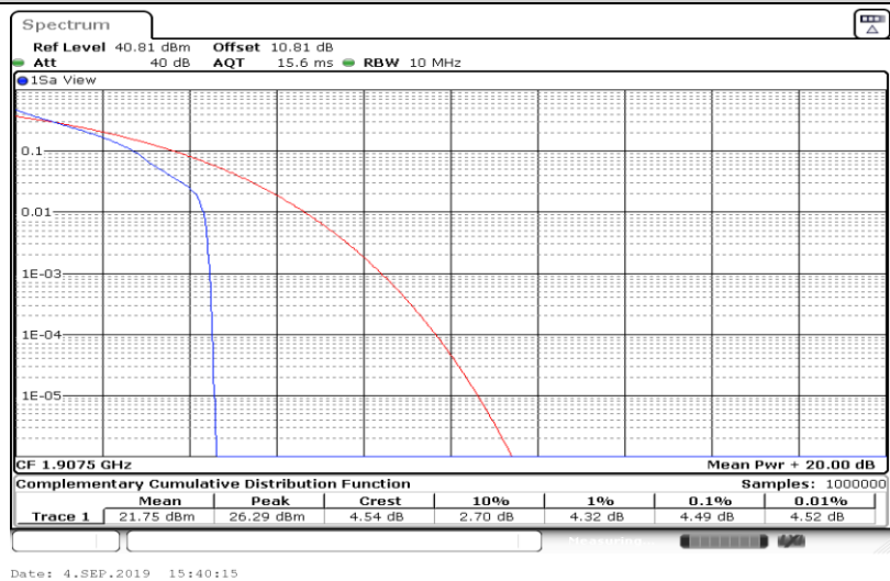
Band2-5MHz-QPSK-19175-25RB#0
