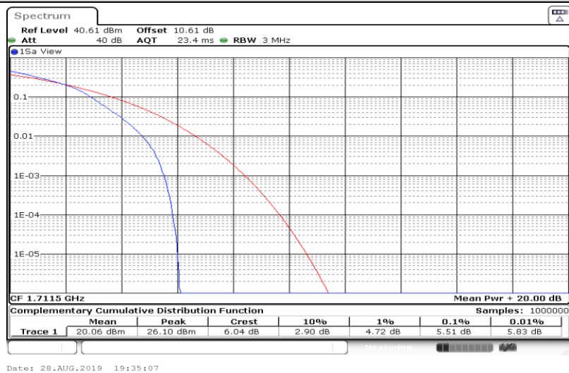
Band4-3MHz-16QAM-20175-1RB#0
