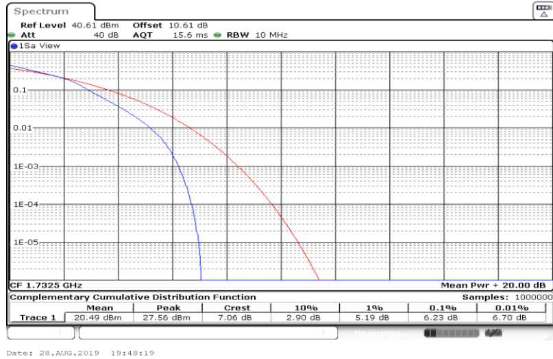
Band4-5MHz-16QAM-20375-1RB#0
