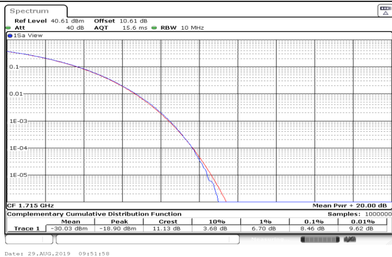
Band4-10MHz-16QAM-20175-1RB#0
