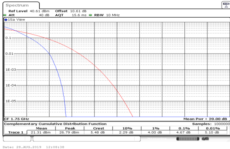
Band4-10MHz-16QAM-20000-1RB#0
