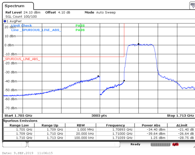
Band66-1.4MHz-QPSK-132665-1RB#0
