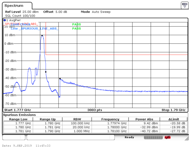
Band66-1.4MHz-16QAM-132665-6RB#0
