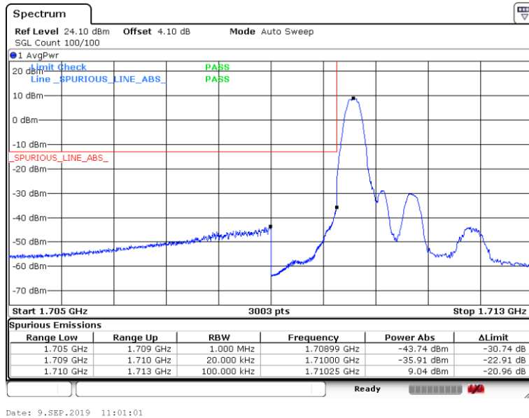
Band66-1.4MHz-QPSK-131979-6RB#0
