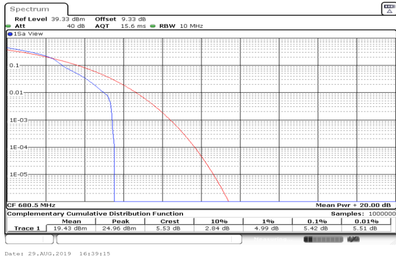
Band71-10MHz-16QAM-133297-49RB#0
