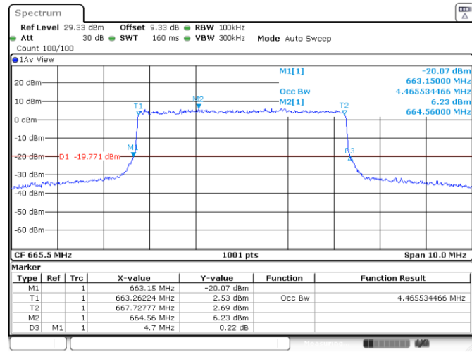
Band71-5MHz-QPSK-133147-25RB#0-4.466
