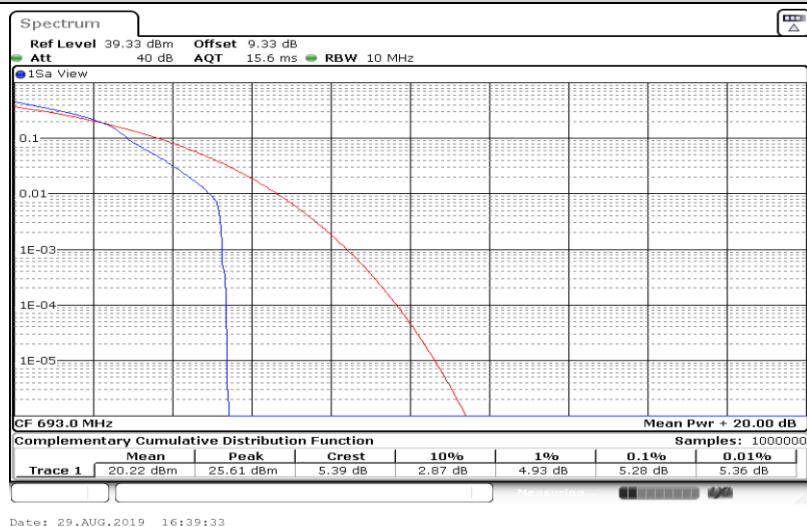
Band71-10MHz-16QAM-133422-49RB#0
