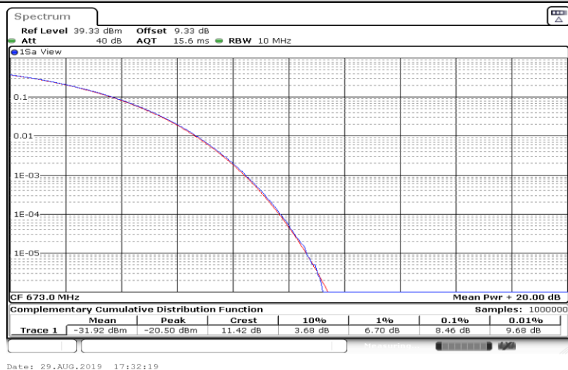
Band71-20MHz-16QAM-133322-1RB#0
