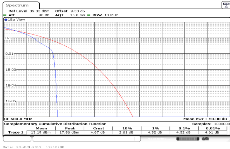
Band71-20MHz-QPSK-133322-100RB#0
