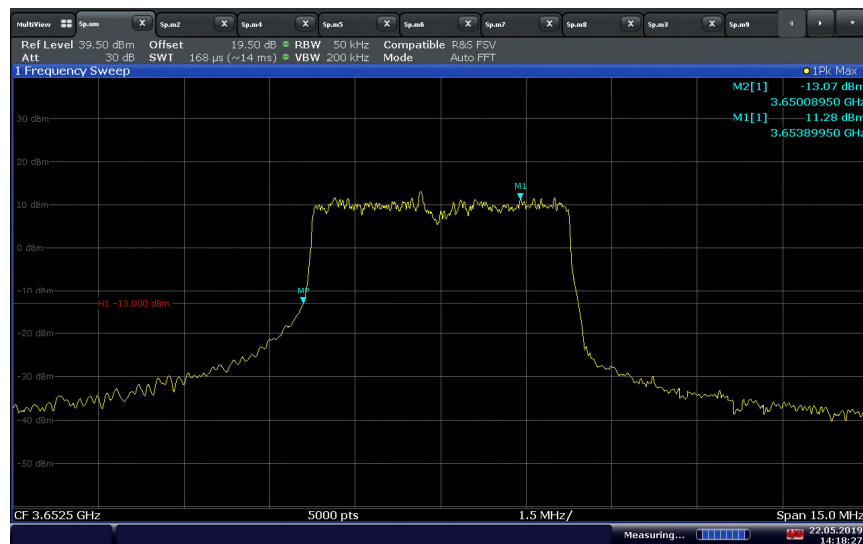
LTE Band 48 (3650-3700 MHz) – QPSK 5 MHz BW Low Channel F_L at Normal Voltage 20°C
