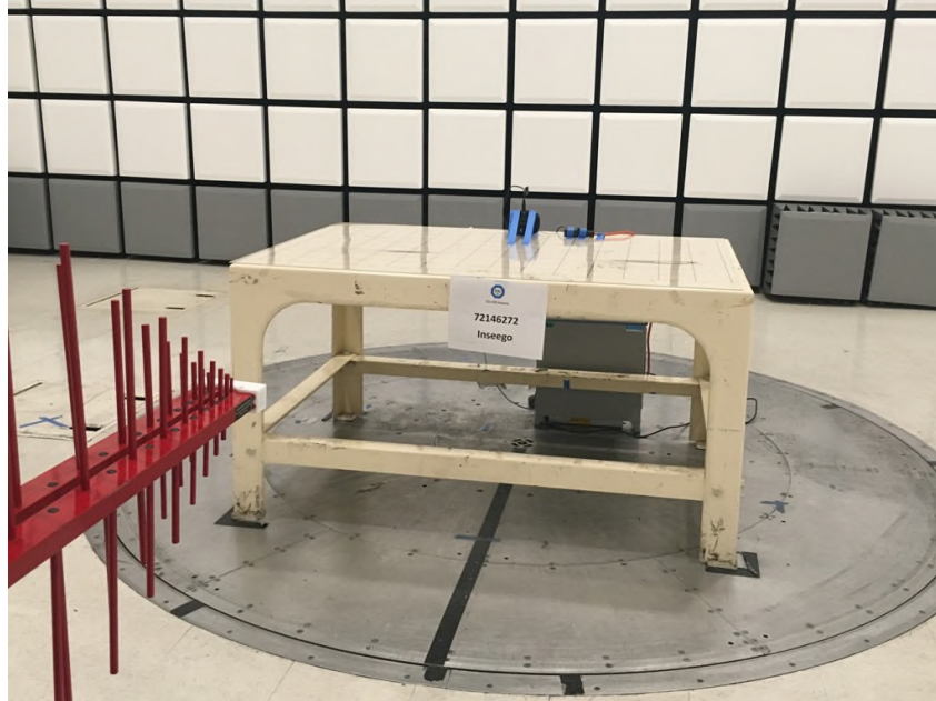
Radiated Emissions Below 1GHz Front (Cell Transmission Mode)
