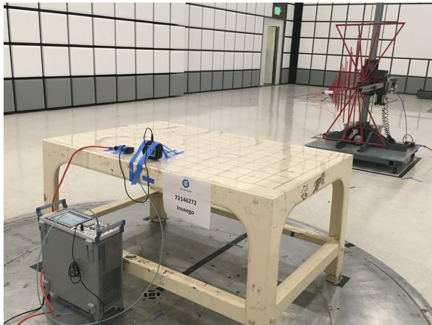
Radiated Emissions Below 1GHz Rear (Cell Transmission Mode)
