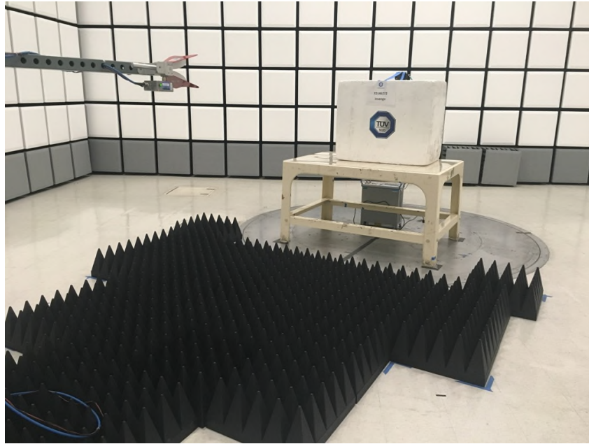
Radiated Emissions Above 1GHz Front (Cell Transmission Mode)
