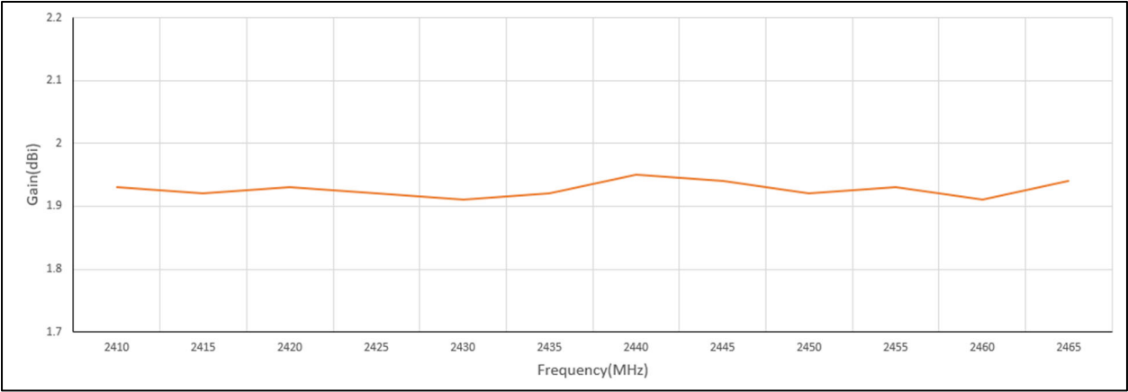
Maximum Gain WiFi ANT W0 2.4GHz (DTS)
