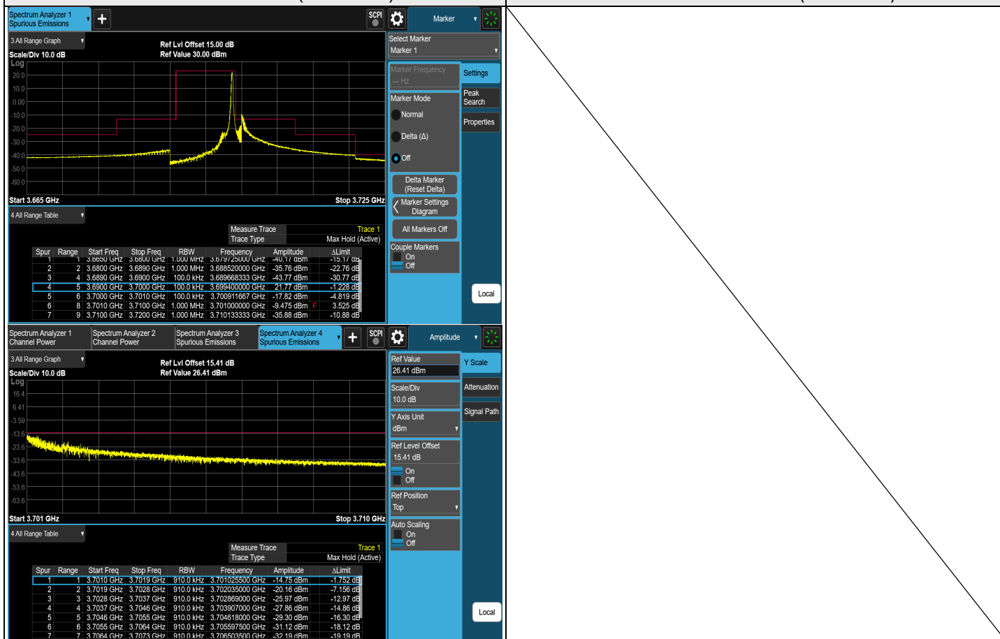
1RB#MAX CH 56690 (3695 MHz)
