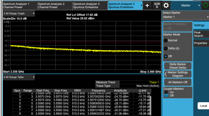
1RB#MAX CH 55265 (3552.5 MHz)
