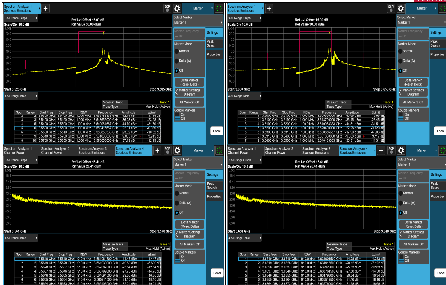
1RB#MAX CH 55290 (3555 MHz)
