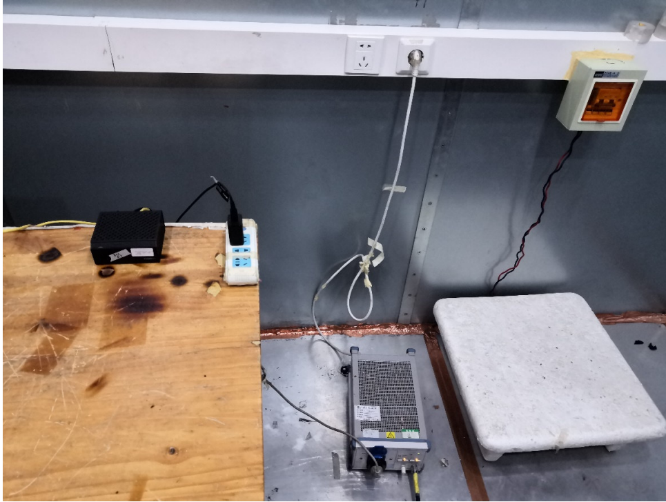
Picture 2: Conducted Emissions Test Setup
