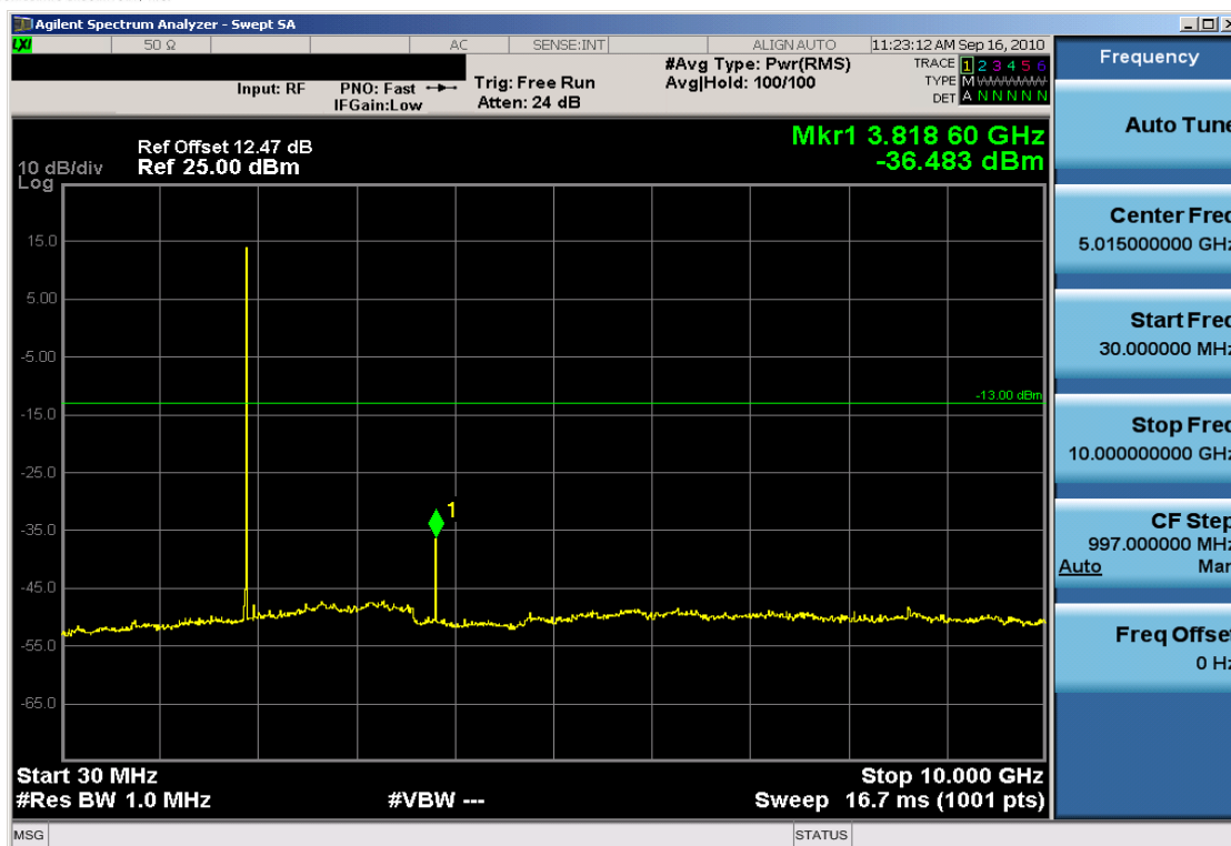
Plot 7-65. Conducted Spurious Plot (PCS CDMA Mode – Ch. 1175)
