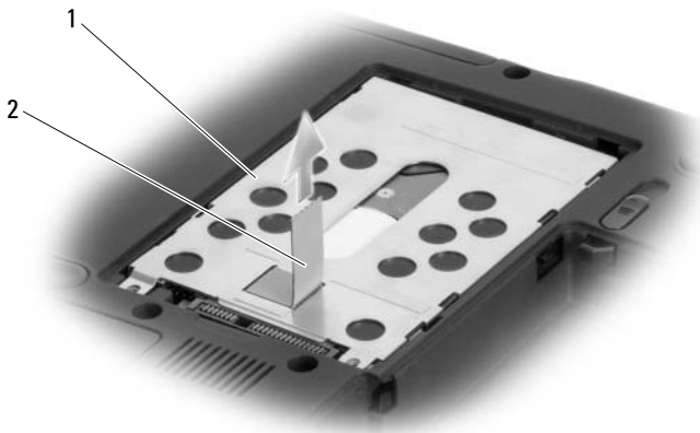
1 hard drive assembly 2 pull-tab
