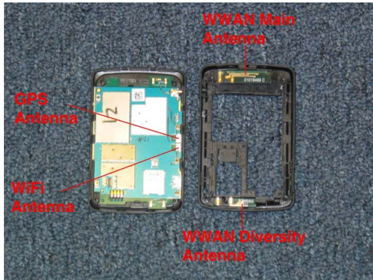
Antenna Locations
