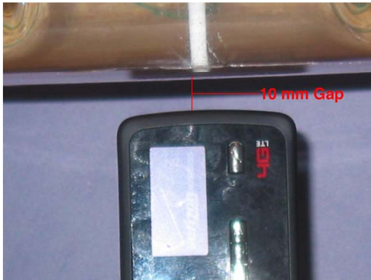
Test Configuration Side E 10 mm Gap
