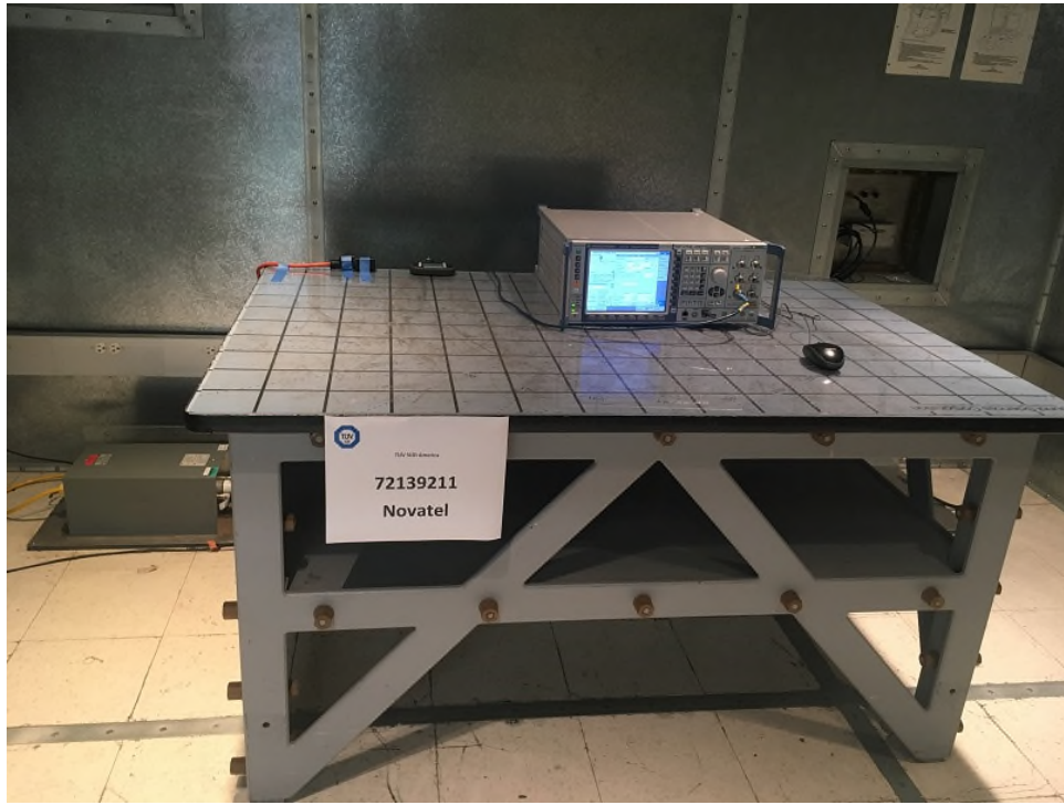
Conducted Testing Front (Cell Transmit Mode)
