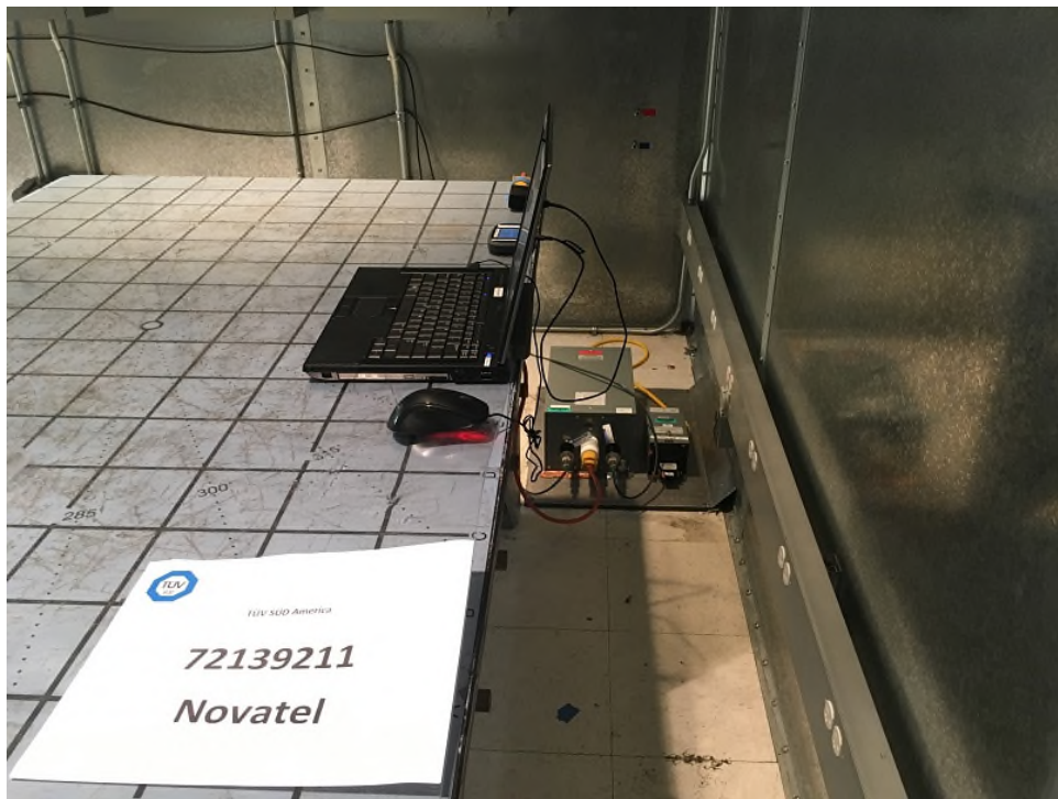
Conducted Testing Rear (WiFi Transmit Mode)
