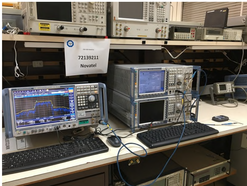
Cell Conducted Testing
