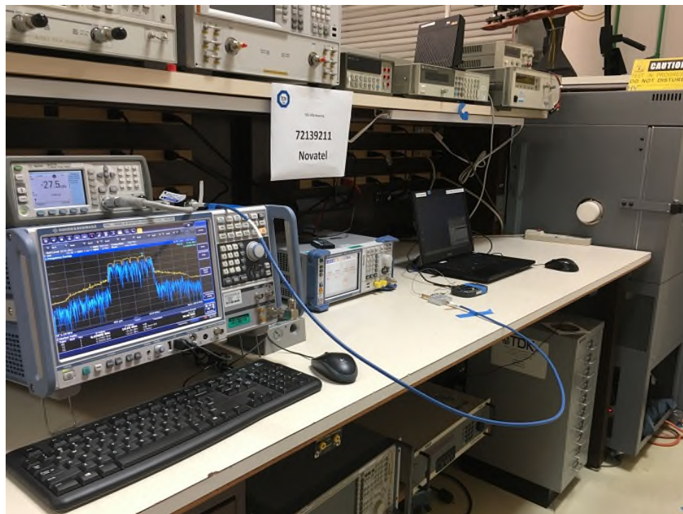
WiFi Conducted Testing
