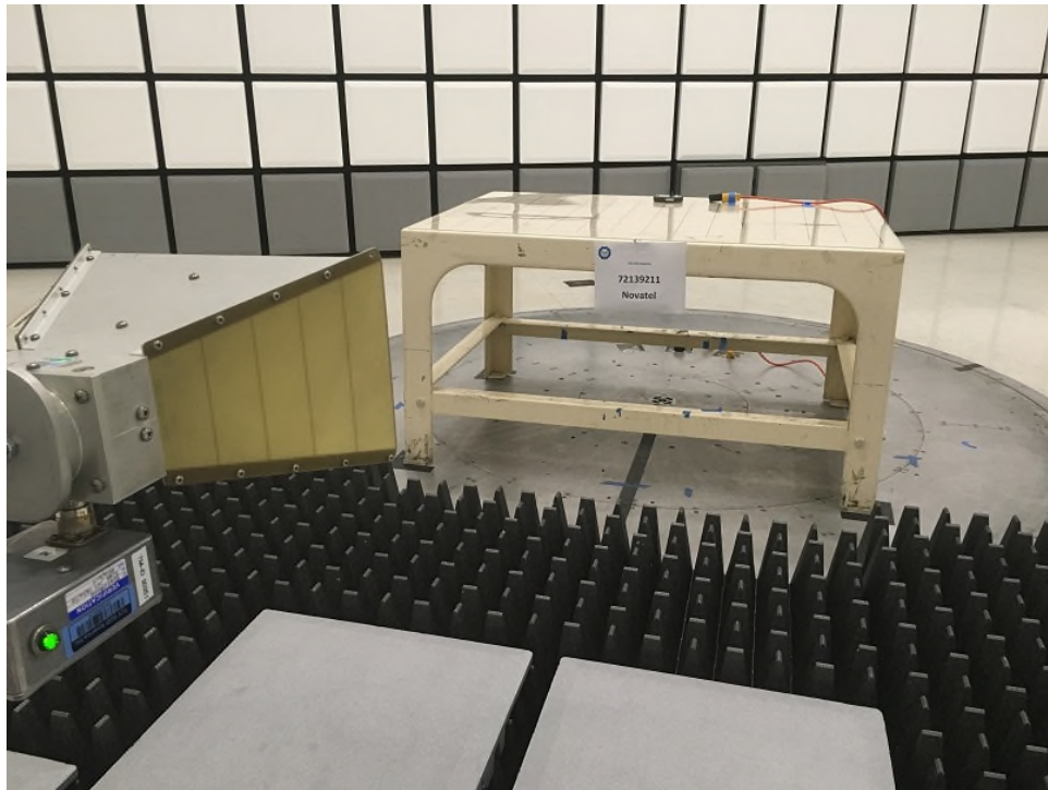
Radiated Emissions Above 1GHz Front (Standby Mode)
