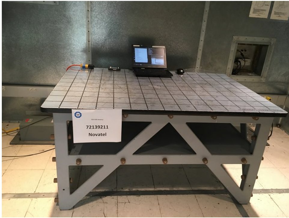
Conducted Testing Front (WiFi Transmit Mode)
