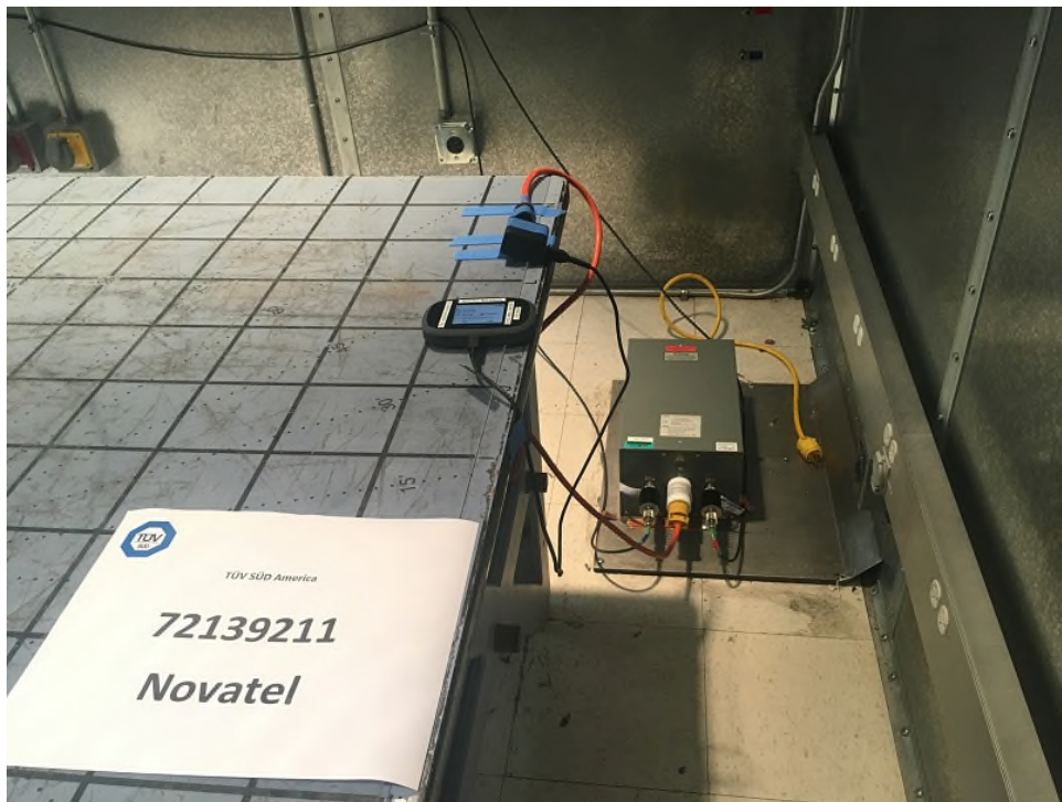
Conducted Testing Rear (Standby Mode)
