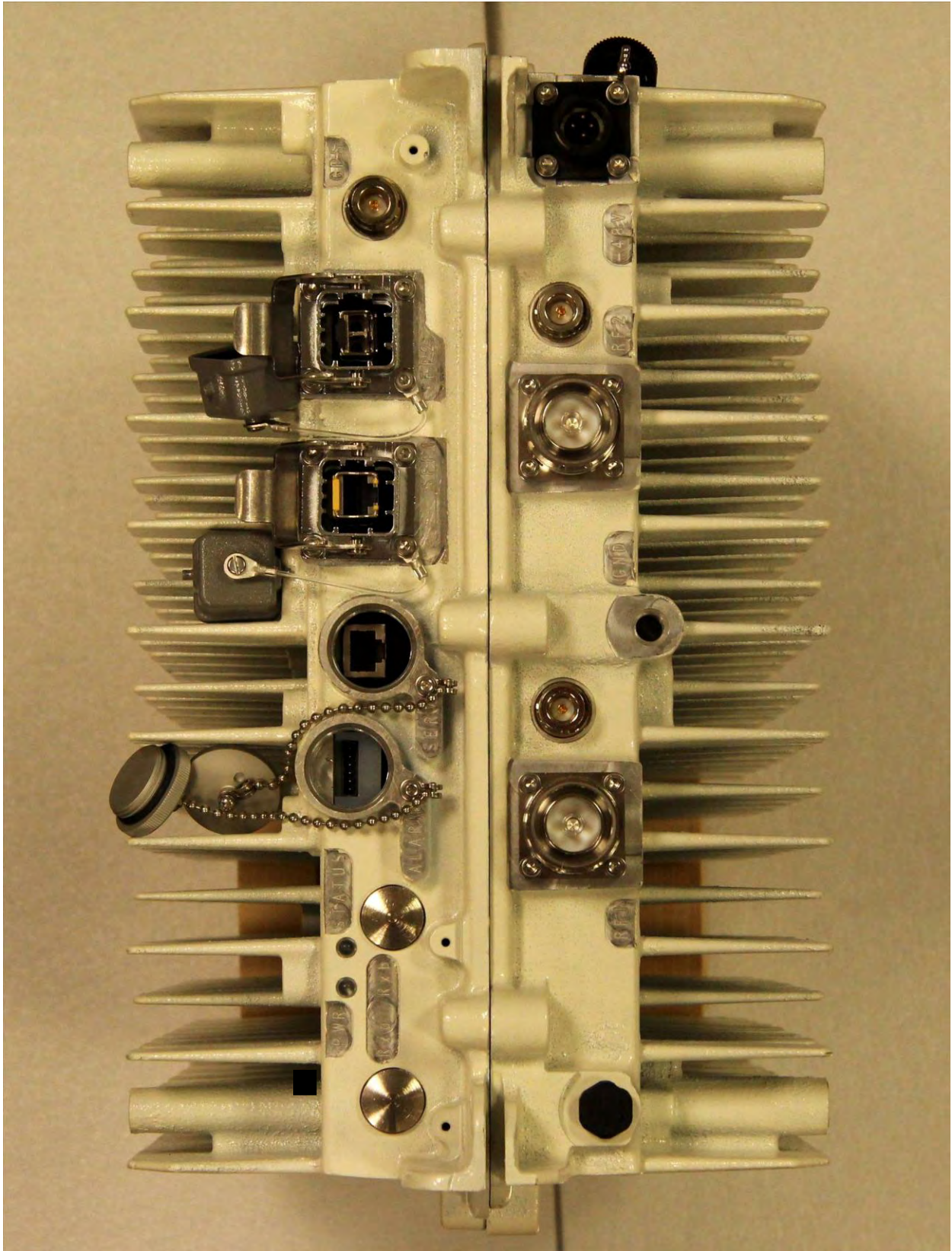
Figure 3: RN2420 External Connectors
