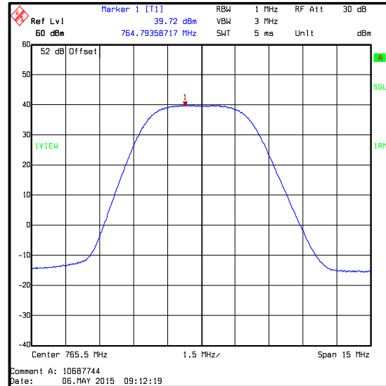
Port RF2
