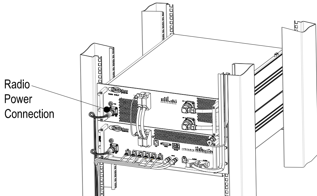
Figure 6-11 : Power Connection to the radio shelf
