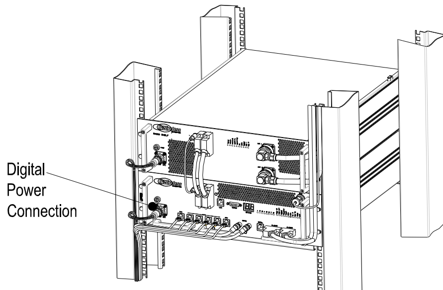
Figure 6-10 : Power Connection to the digital shelf
