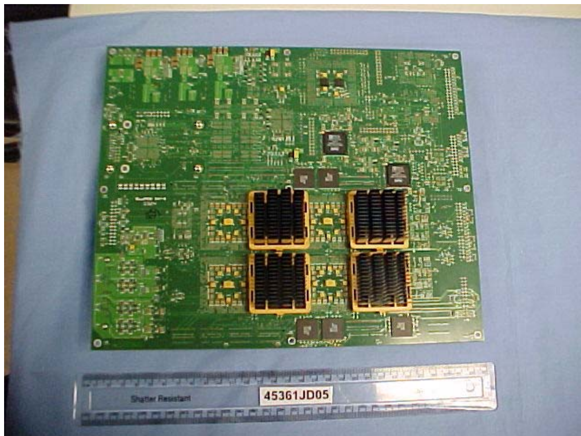
DN PCB3 Side 2
