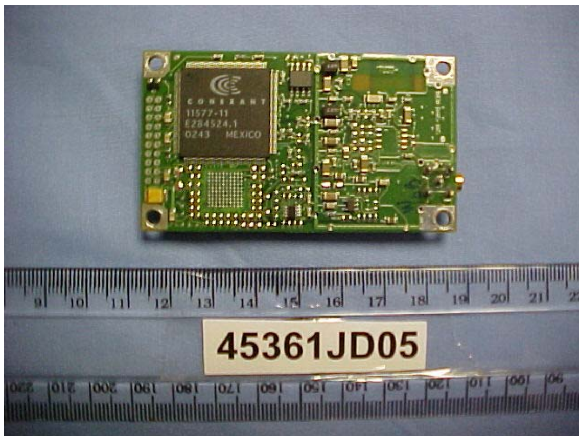
DN PCB2 Side 2
