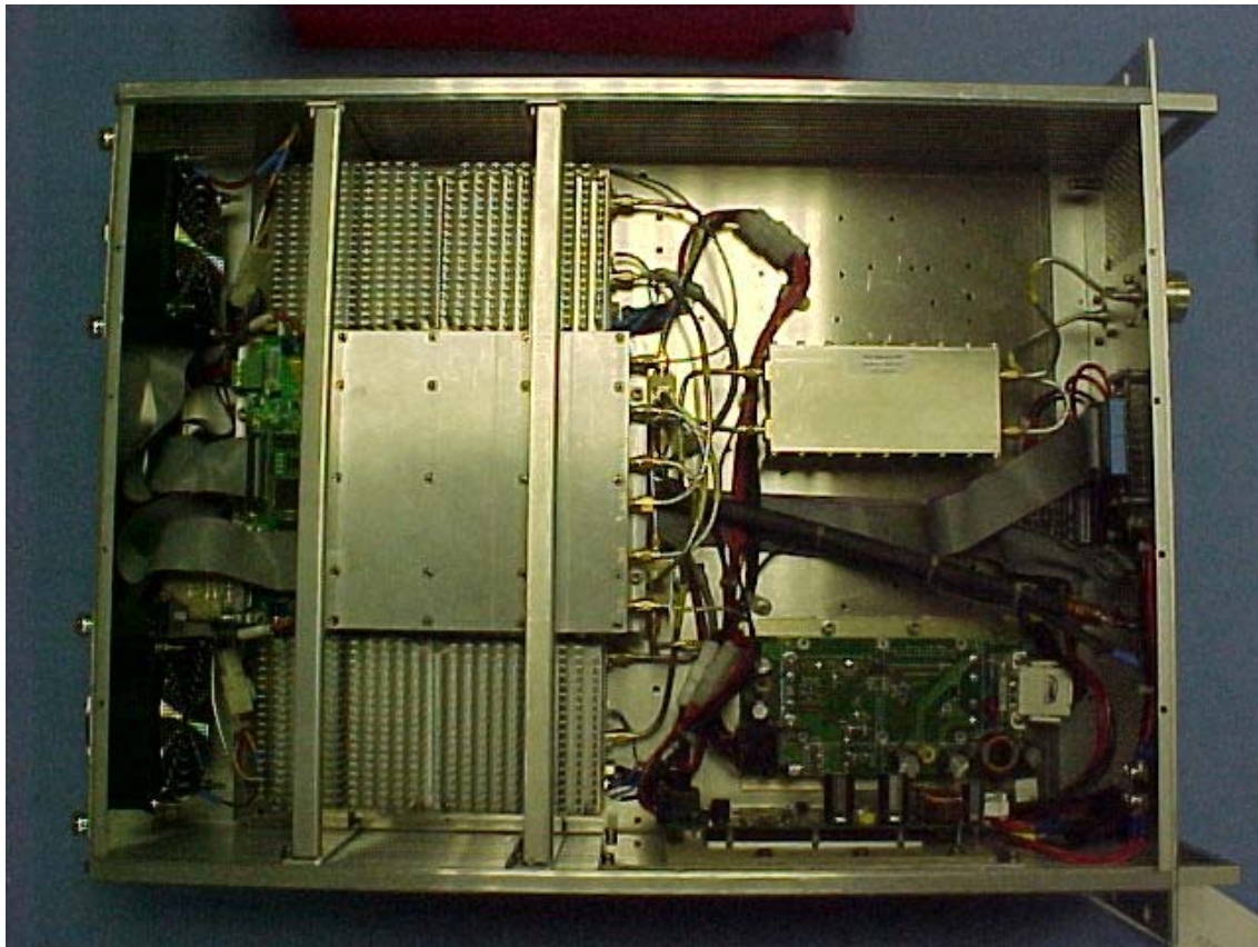
DZ Top Cover Removed
