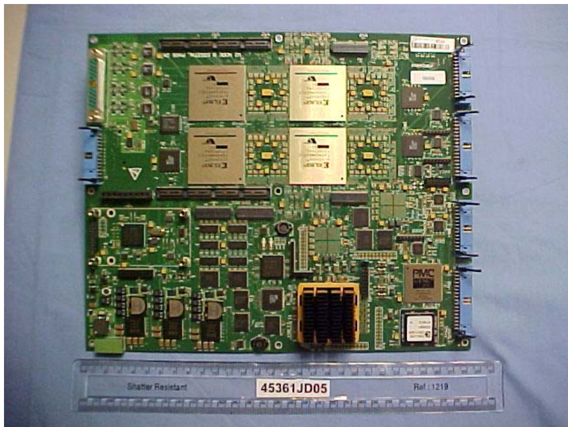
DN PCB3 Side 1
