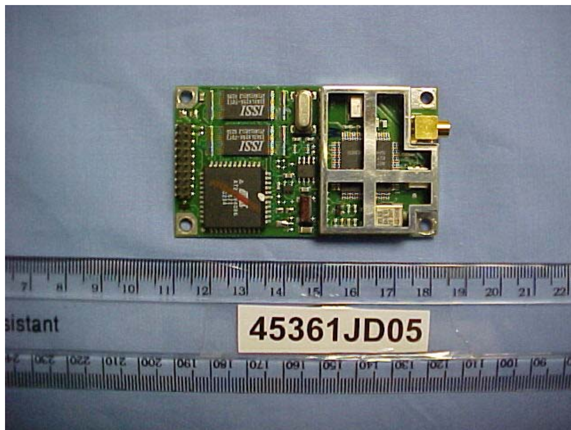
DN PCB2 Side 1
