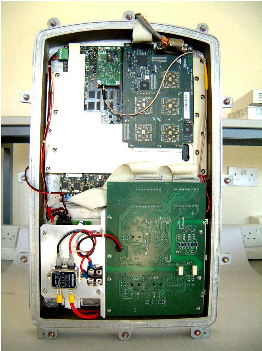
PHT/44493/001 V2 Internal Digital Section
