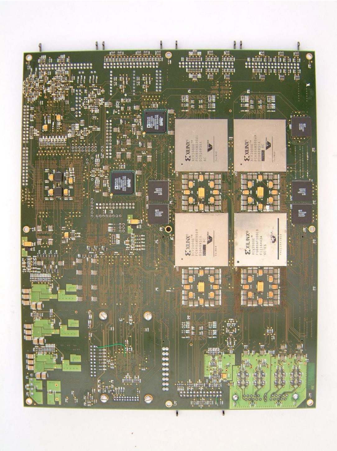
PHT/44493/005 Digital Board Rear
