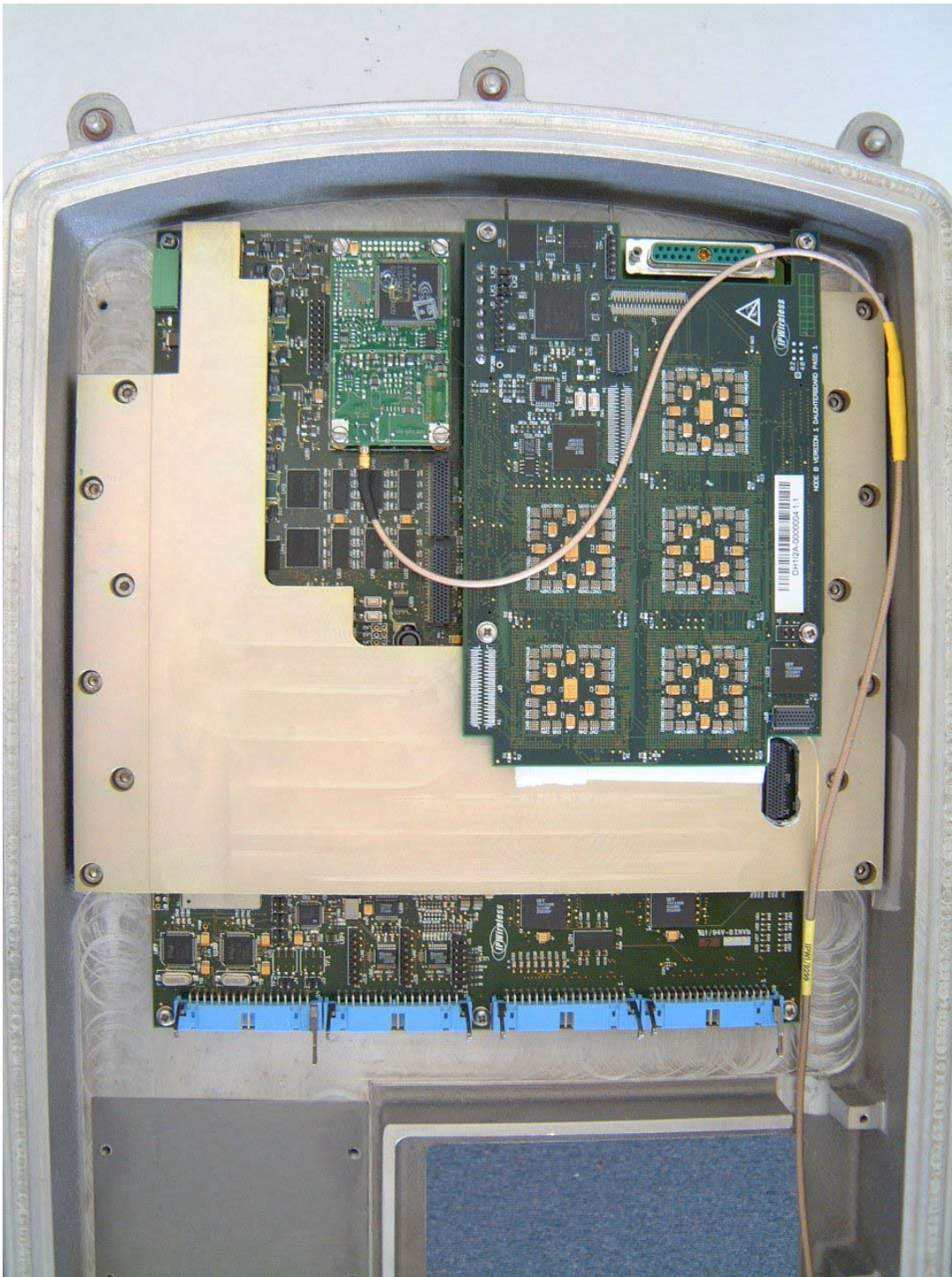
PHT/44493/003 Digital Board with Daughter Board and Heatsink
