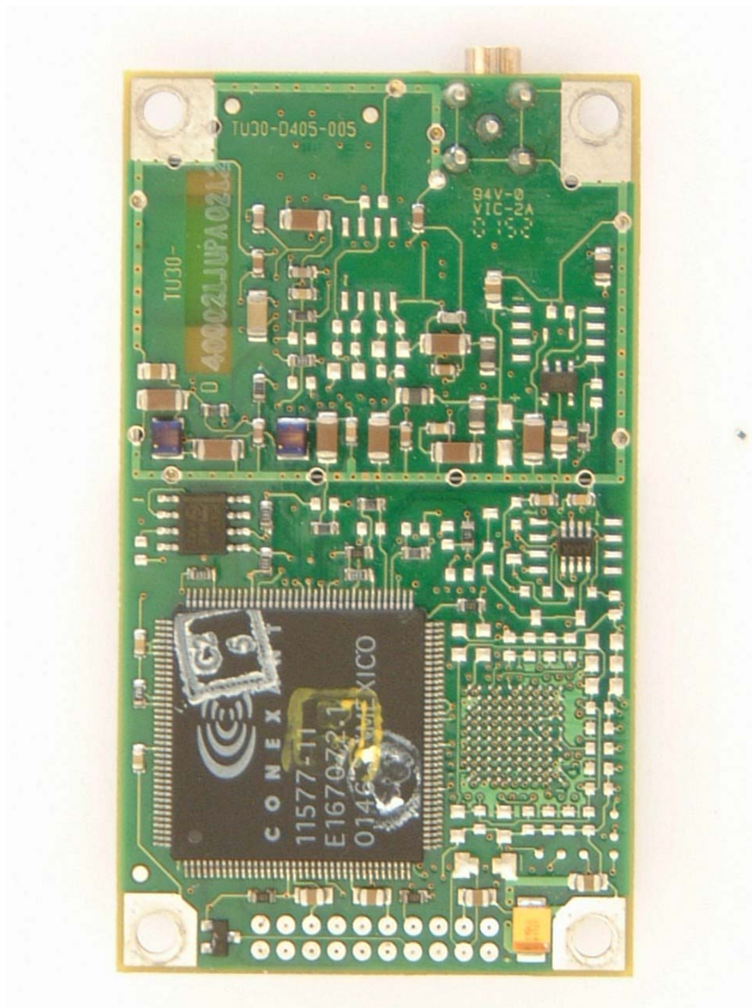
PHT/44493/010 GPS Board Rear
