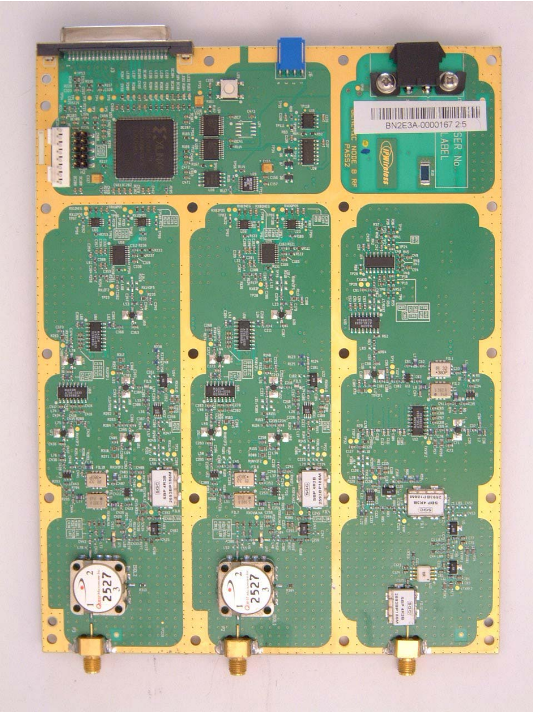
PHT/44493/022 Radio Board Top
