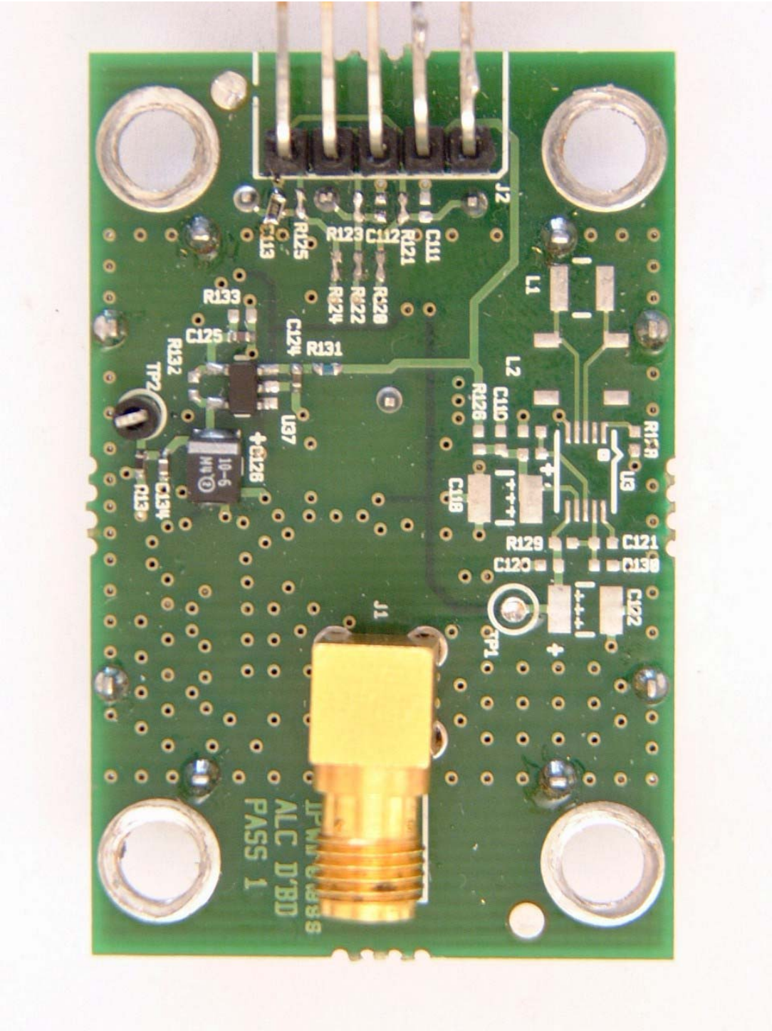
PHT/44493/030 ALC Board Bottom
