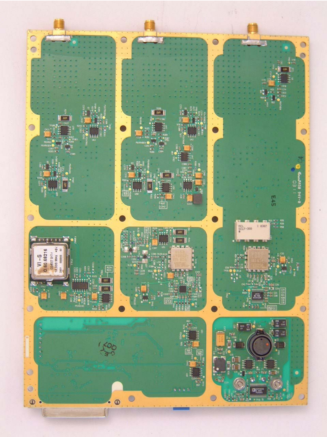
PHT/44493/021 Radio Board Bottom
