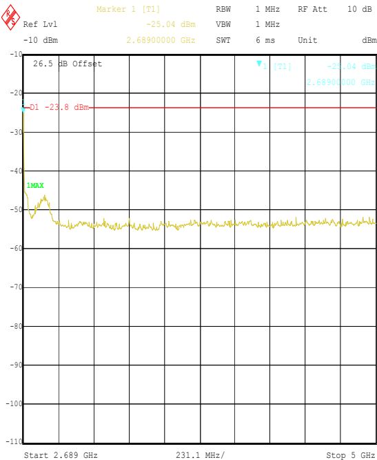
Title: IPWireless EUT; FD, FCC P15/21/74, Conducted Spurious Comment A: 45219JD01 Top Channel 7.68 Mcps. 004 Date: 5.FEB.2004 14:48:32
