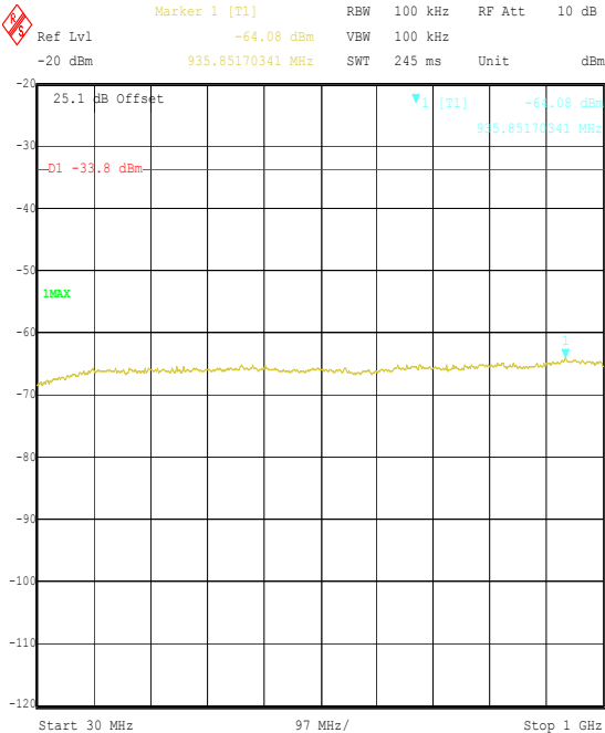
Title: IPWireless EUT; FD, FCC P15/21/74, Conducted Spurious Comment A: 45219JD01 Top Channel 7.68 Mcps. 002 Date: 5.FEB.2004 14:36:30
