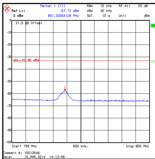
16QAM / 1 Resource Block (25 offset)
