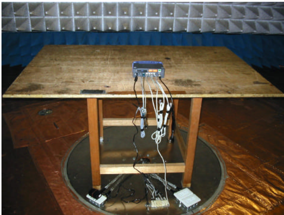
Rear View of the Test Configuration Intentional
