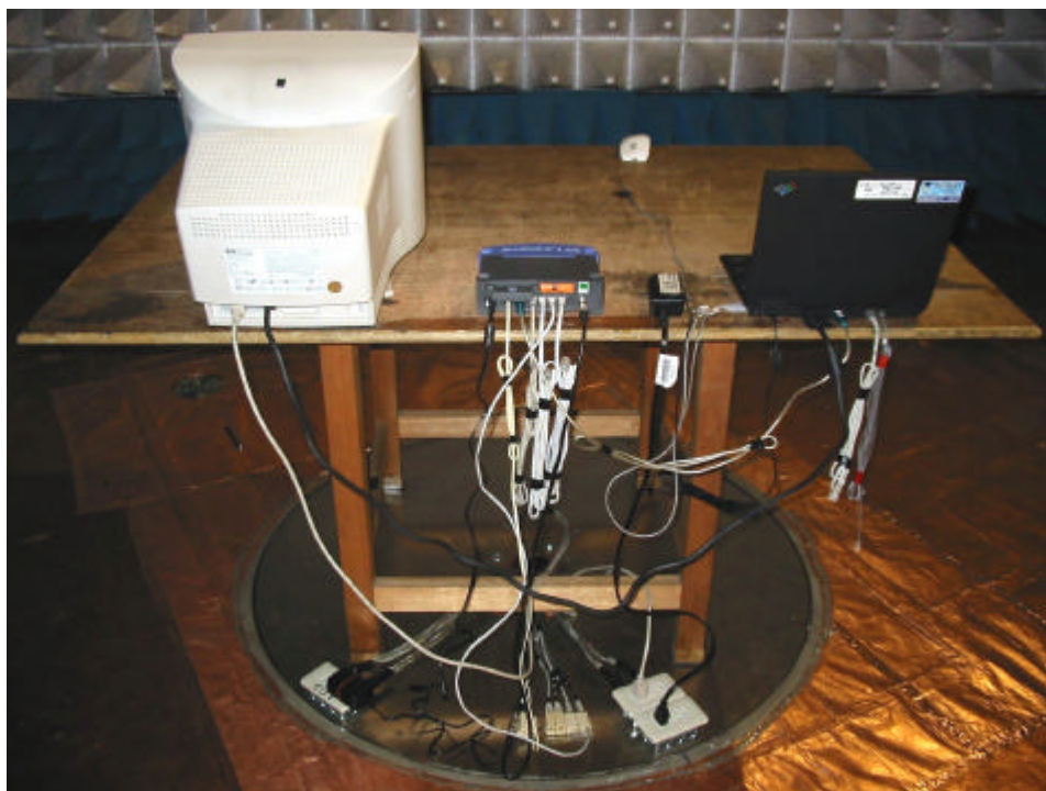
Rear View of the Test Configuration Unintentional
