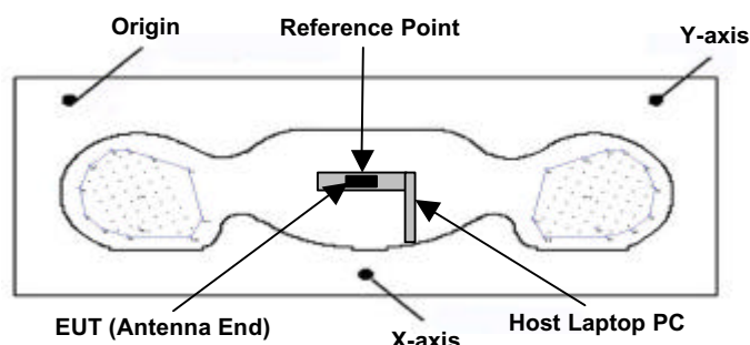
Figure 2. Phantom Reference Point & EUT Positioning Left Side of Laptop PC - EUT Antenna Side
