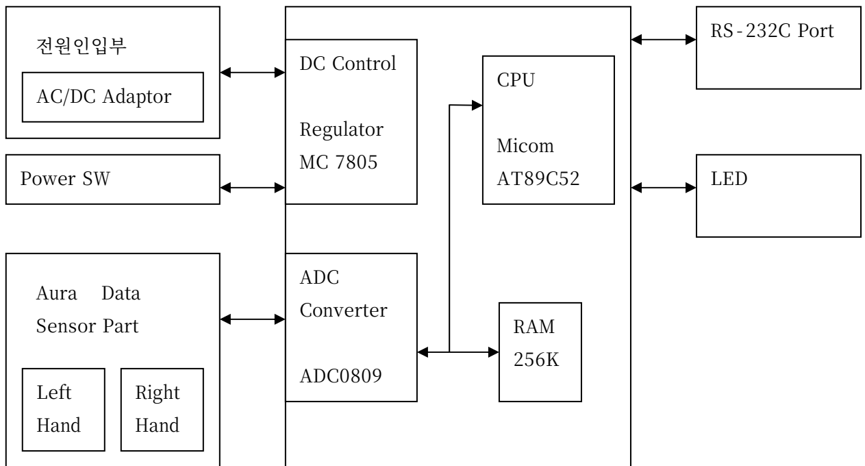
AuraCom Block Diagram
