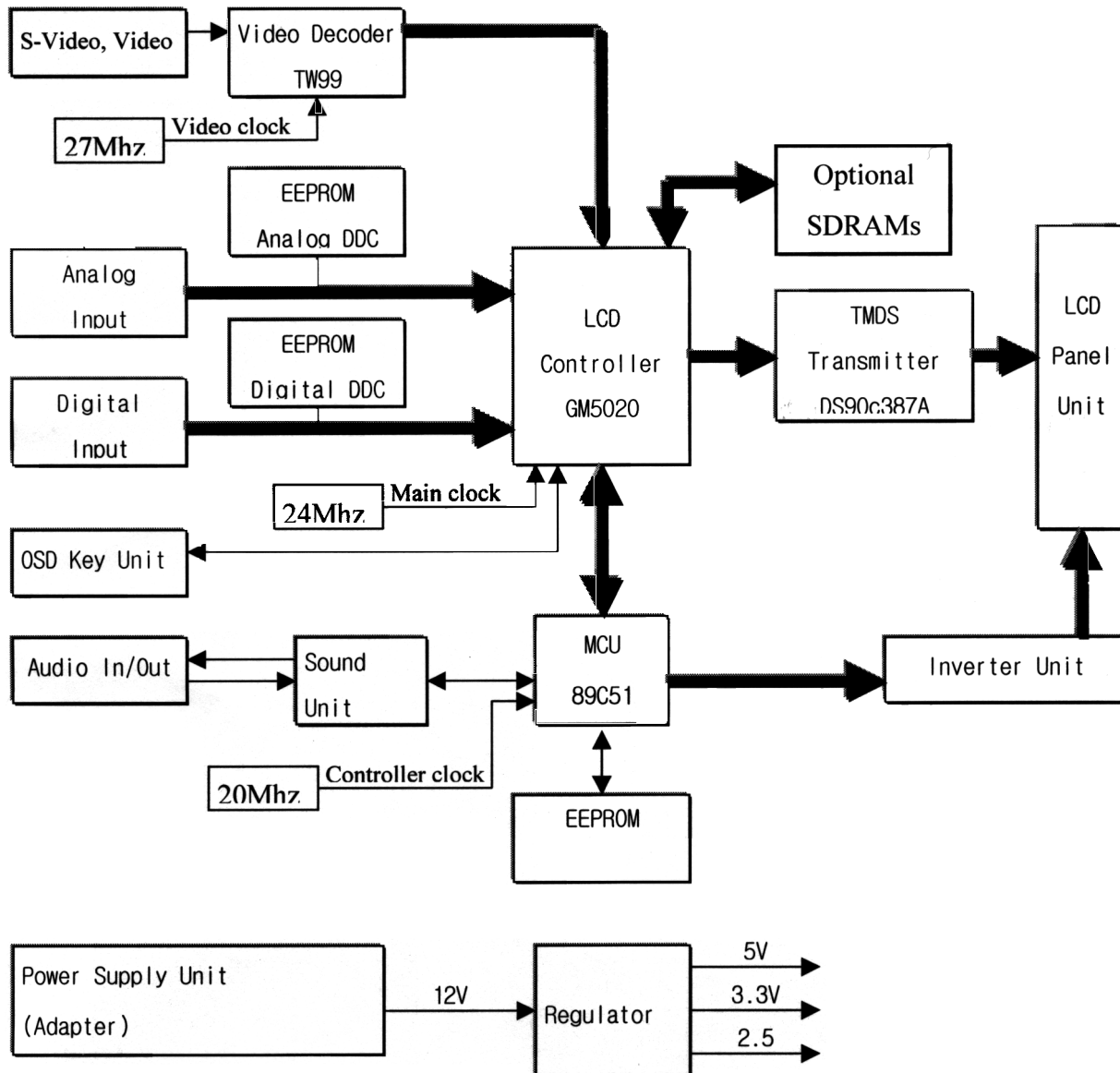
Figure 6 : Block diagram
