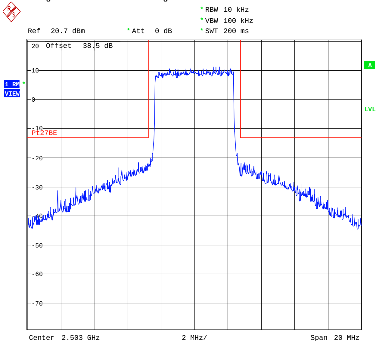
Figure 7 Lower Band Edge OFDM mode
