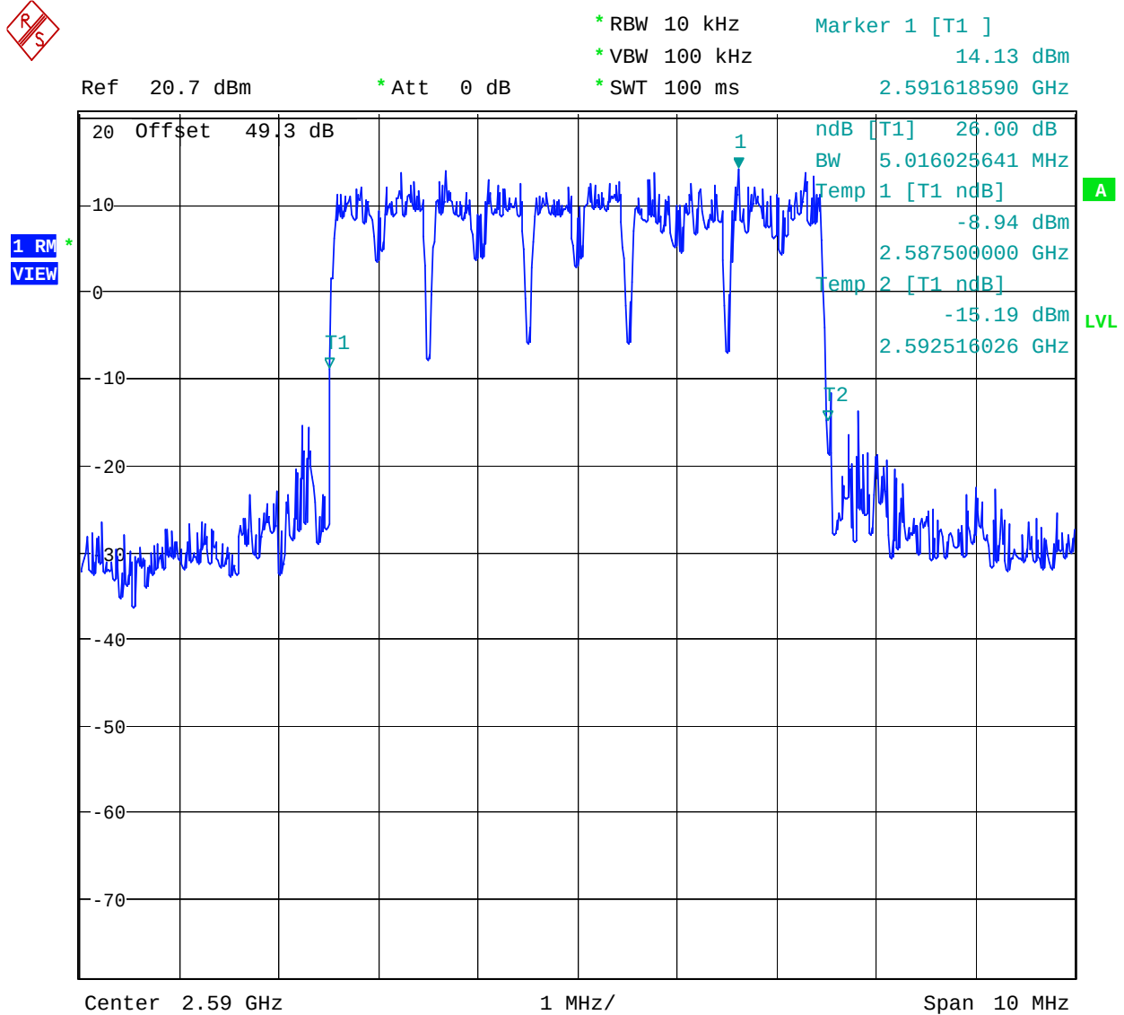
Figure 2 2.590 GHz Navini Mode
