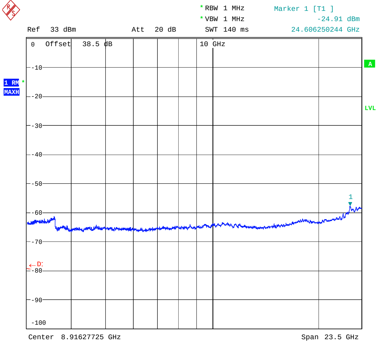
Figure 12 Antenna Conducted Spurious – Navini mode – 2.59 GHz
