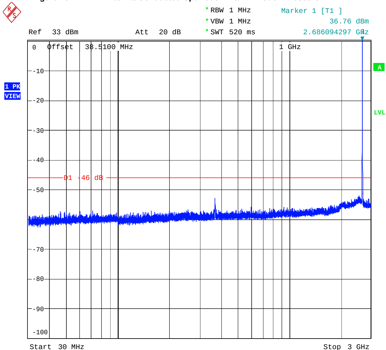
Figure 15 Antenna Conducted Spurious – Navini mode – 2.6835 GHz
