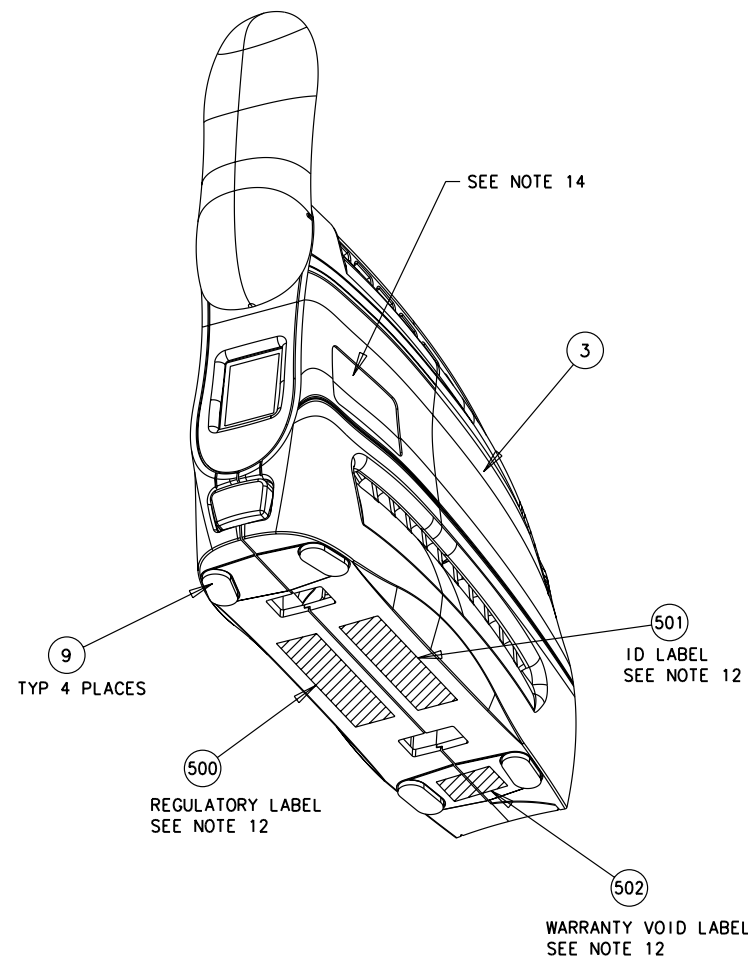
DETAIL "H"
