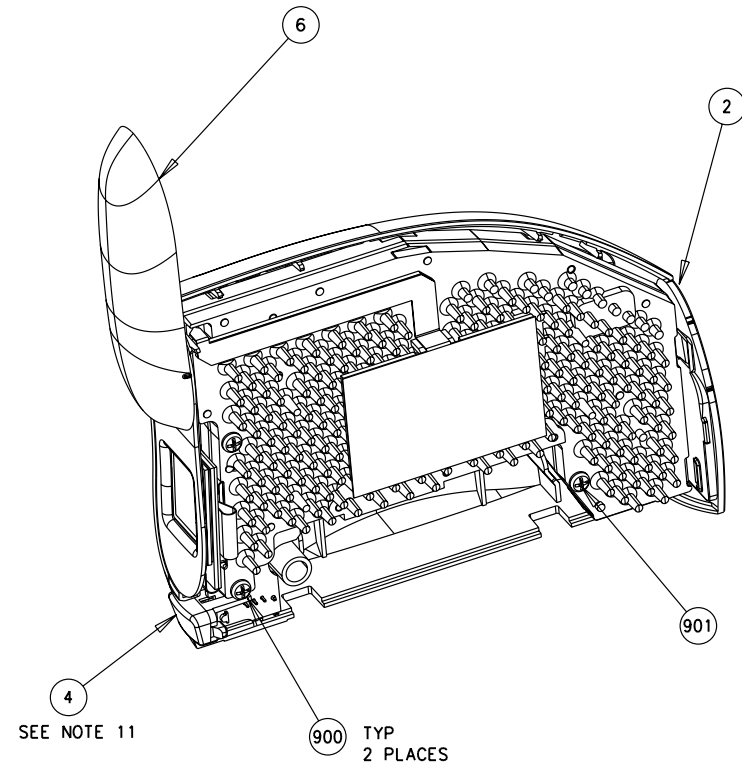
DETAIL "G"
