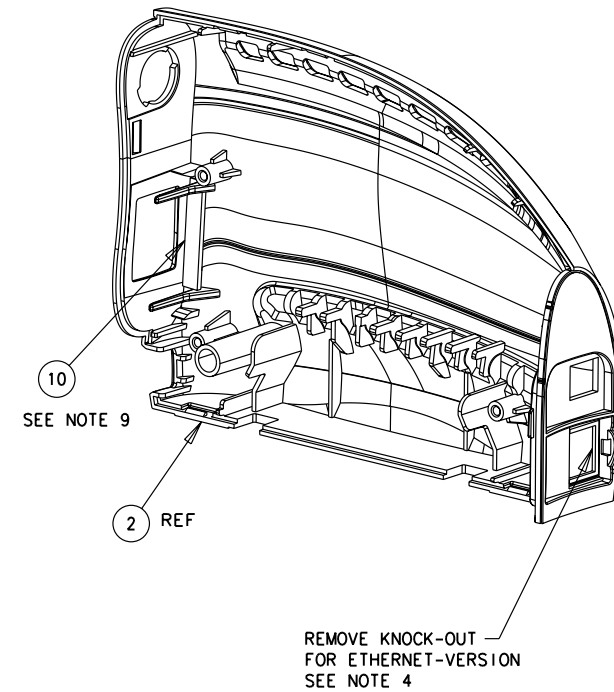
DETAIL "B"
