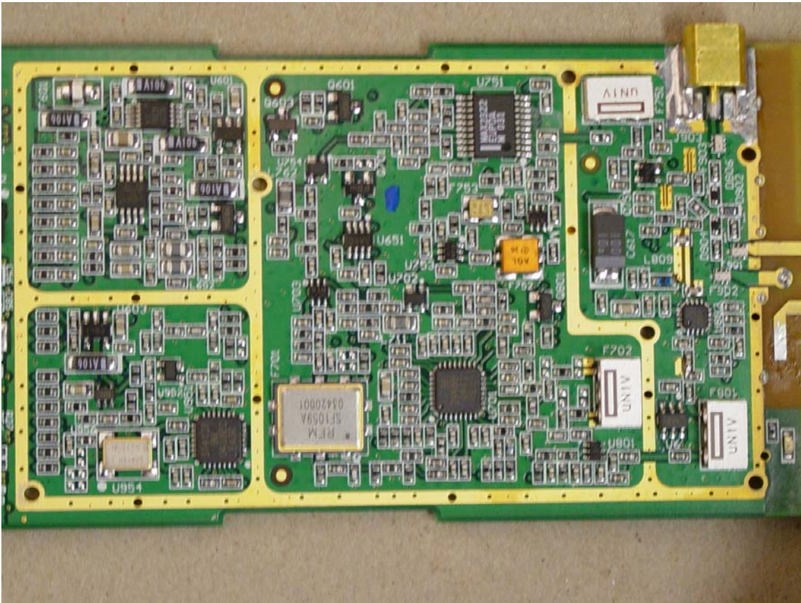
PCMCIA Top Side (under shields)
