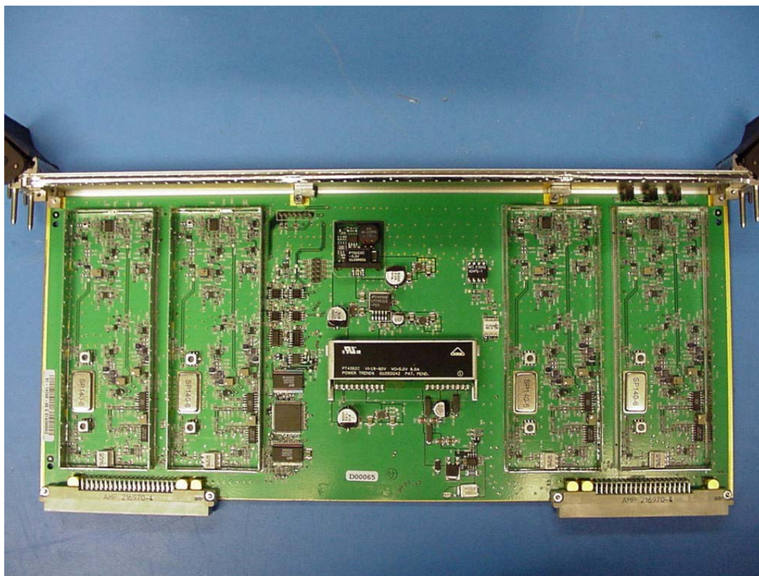
IF Card
