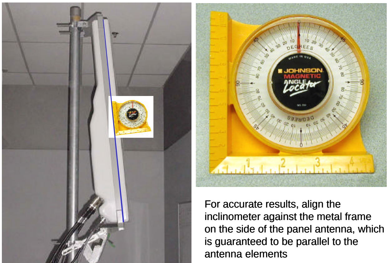
Figure 32: Measuring Antenna Downtilt
