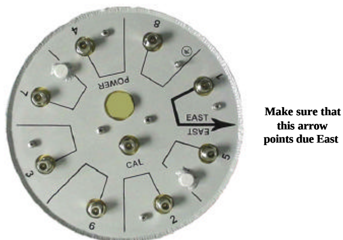
Figure 30: Bottom of an Omni Antenna Showing Correct Orientation
