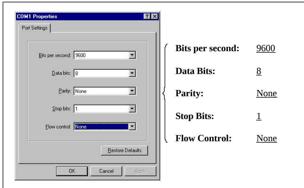
Figure 49: COM1 Properties
