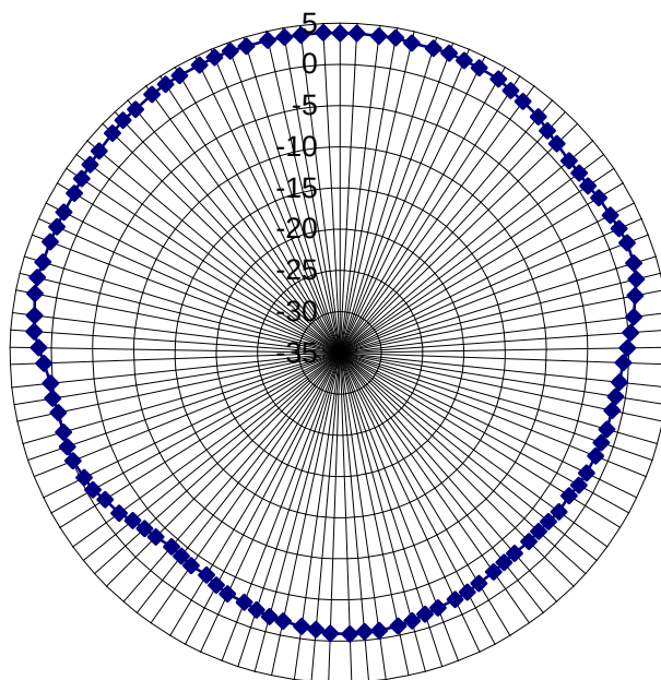
3.8dBi MMDS BroadBeam Directional CPE antenna
